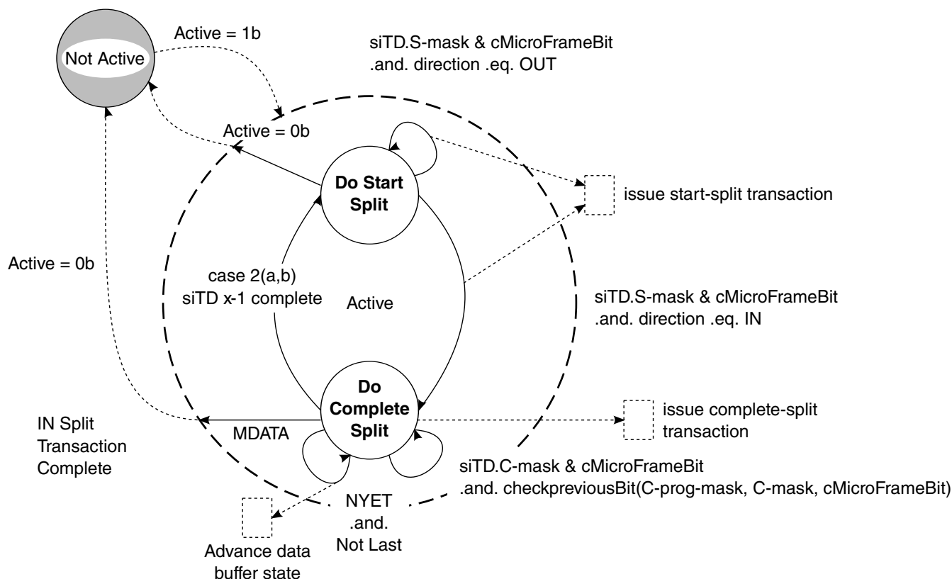
Figure 42-26. Split Transaction State Machine for Isochronous
