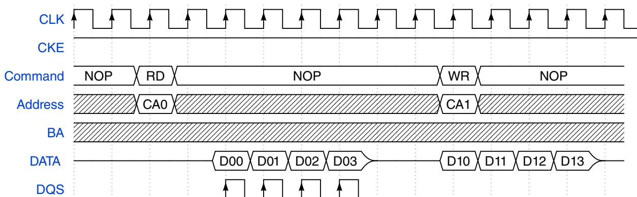
Figure 25-19. SDRAM Read-to-Write access (CL=2)
