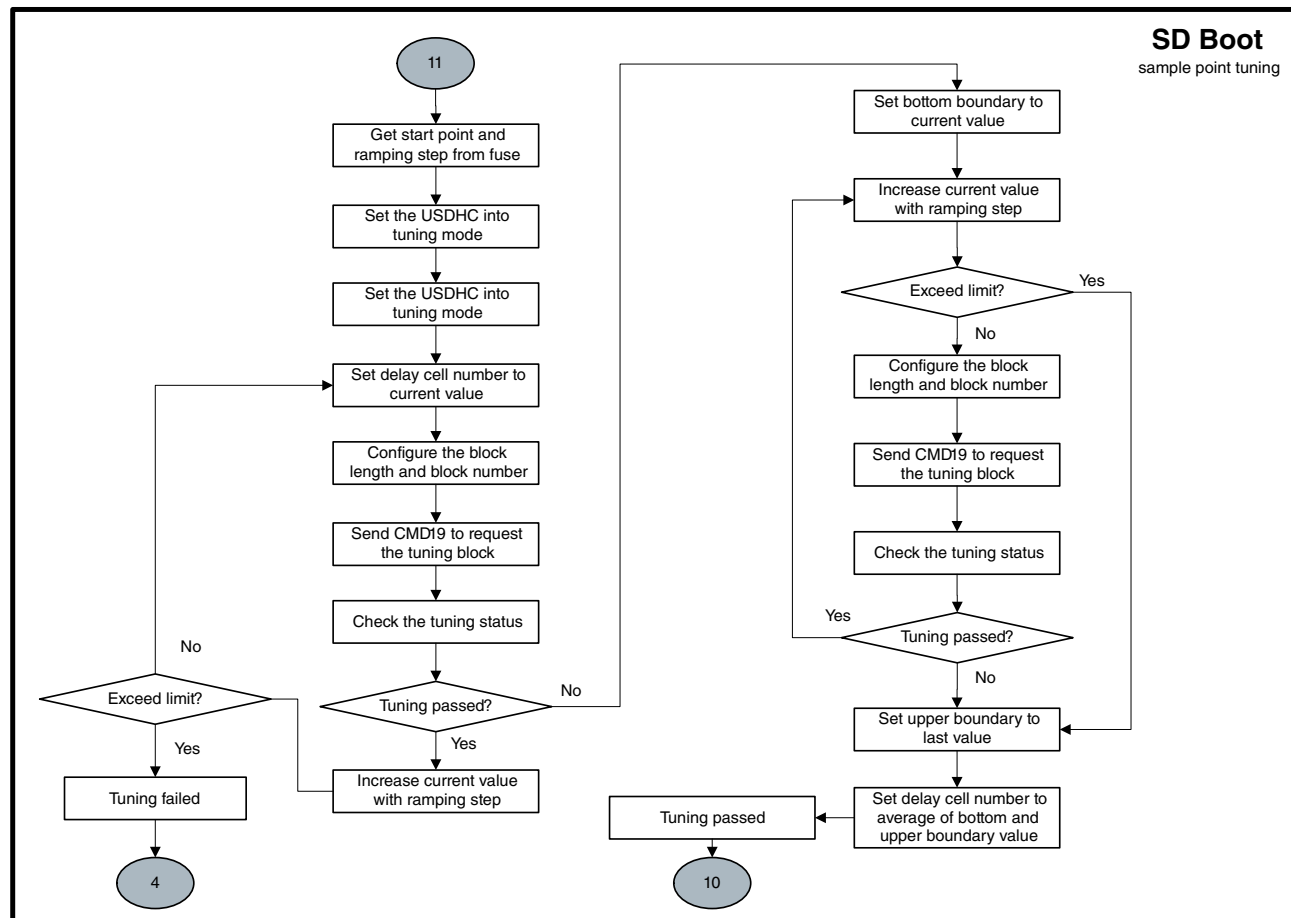
Figure 9-12. Expansion device boot flow (6 of 6) i.MX RT1050 Processor Reference Manual, Rev. 4, 12/2019
