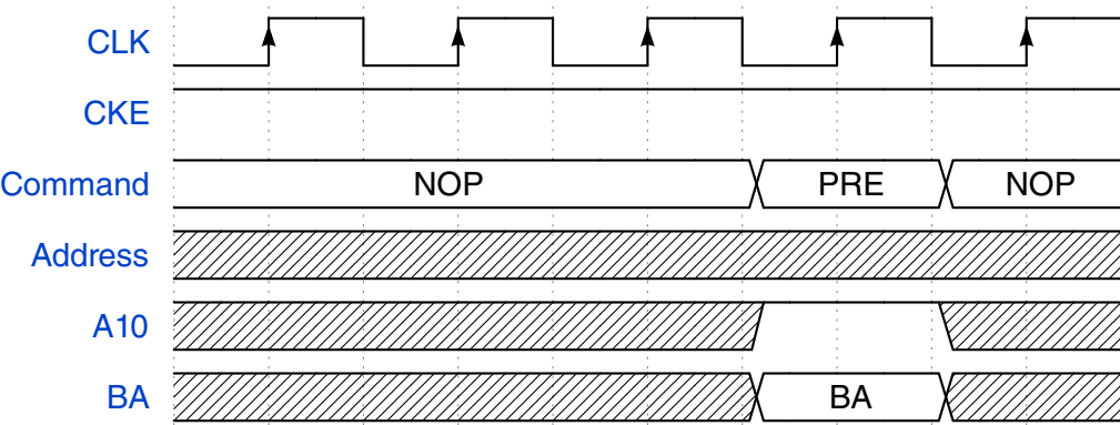
Figure 25-7. IP command - SDRAM PRECHARGE ALL
