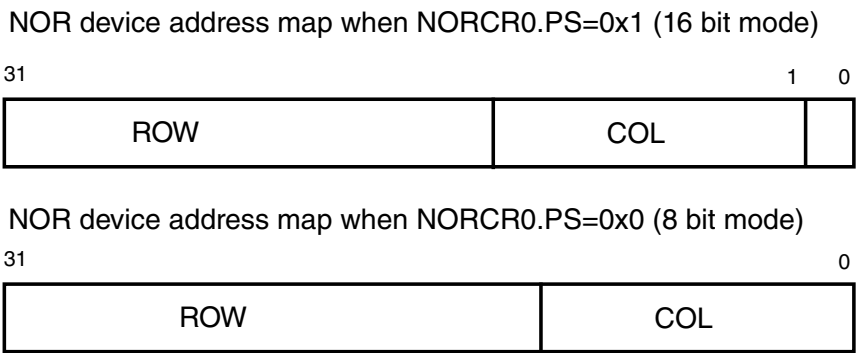
Figure 25-47. NOR Flash Address Map
