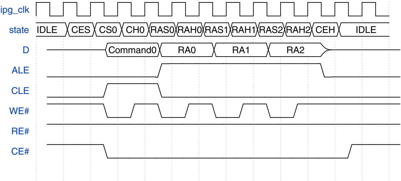
Figure 25-32. NAND Flash access Address type - Three Byte Row Address
