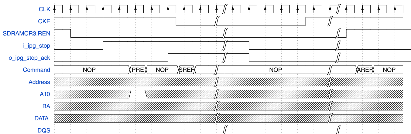
Figure 25-26. Stop mode Enter and Exit- SDRAM
