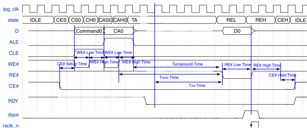
Figure 25-38. NAND Flash access command type - Command + Address + Read Phase
