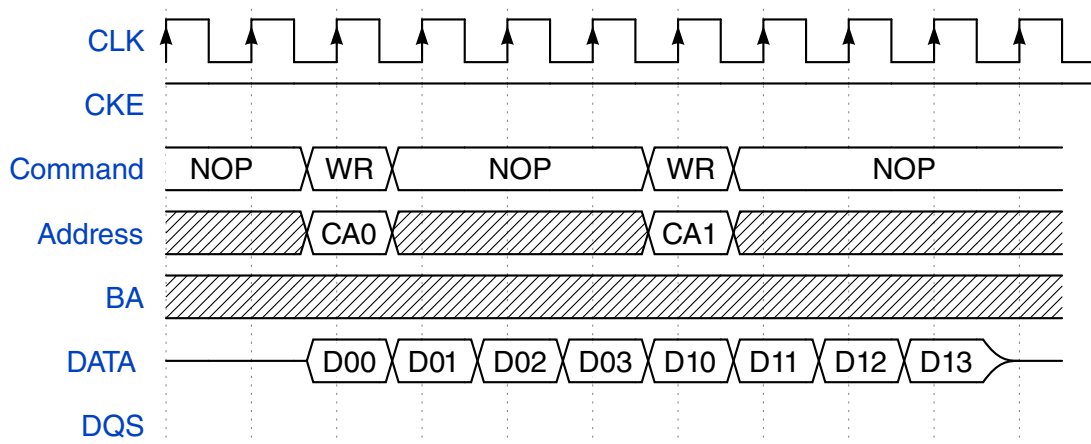
Figure 25-21. SDRAM Write-to-Write access
