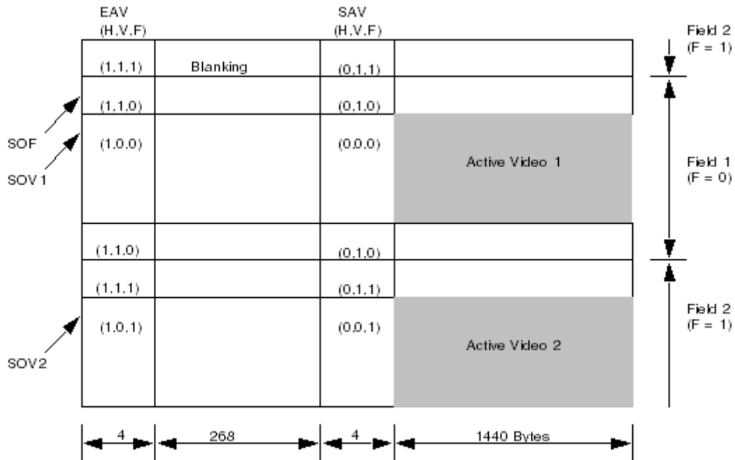
Figure 34-2. CCIR656 Interlace Mode (PAL)
