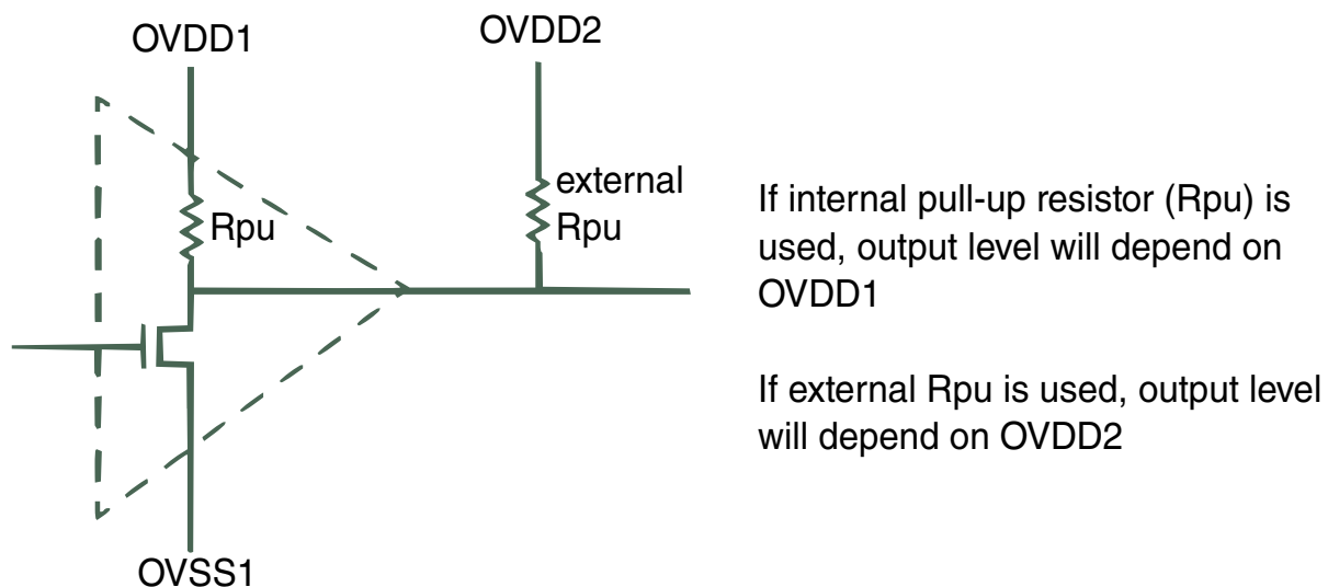
Figure 12-8. Output buffer in open drain mode
