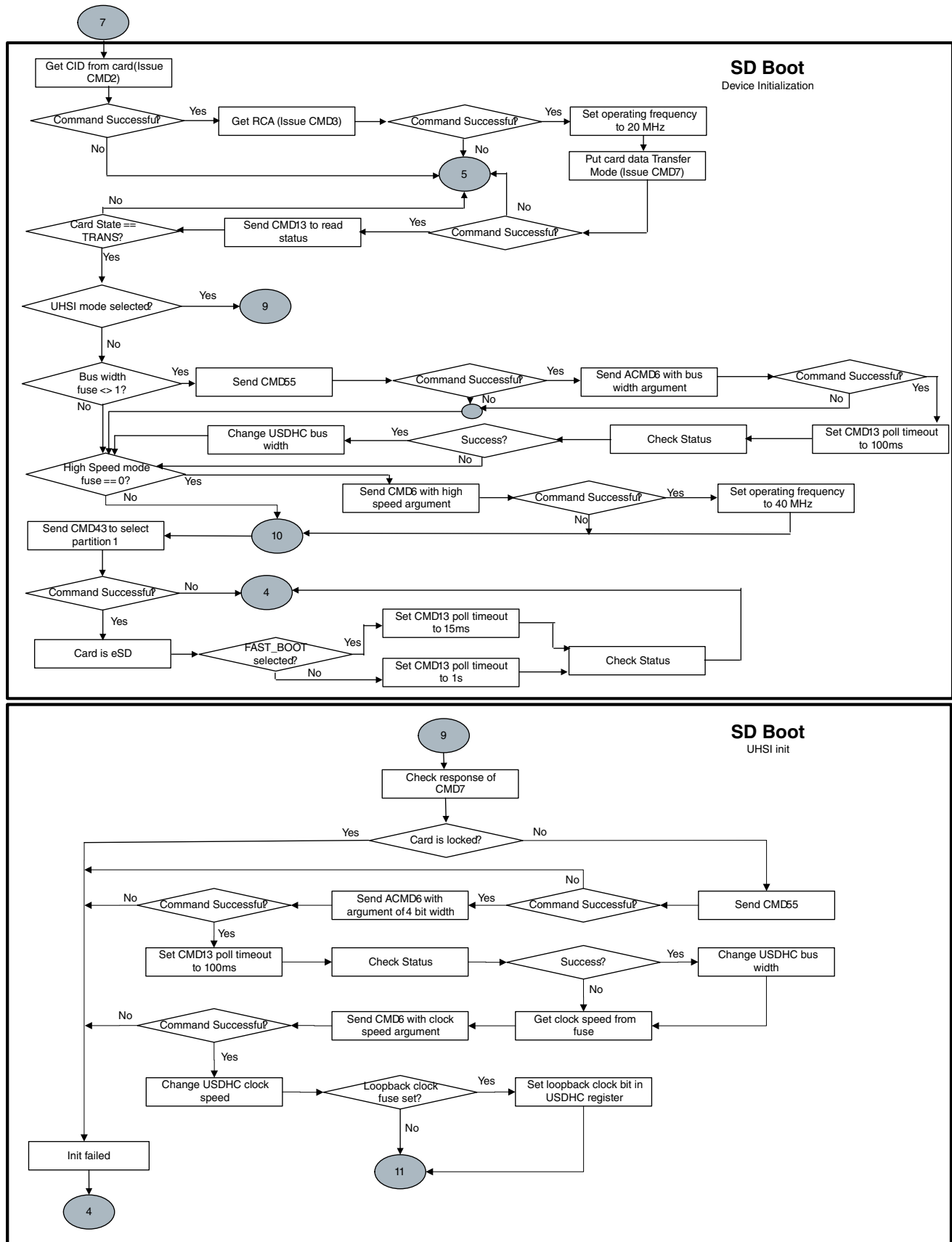
Figure 9-10. Expansion device (MMCSD/eSD/SDXC) boot flow (4 of 6) i.MX RT1050 Processor Reference Manual, Rev. 4, 12/2019
