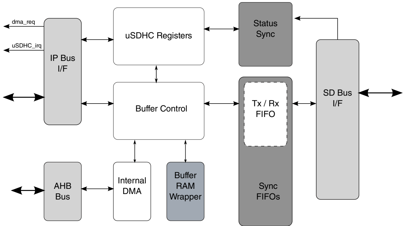
Figure 26-3. uSDHC Buffer Scheme
