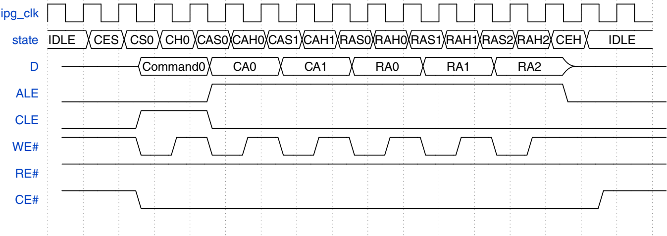
Figure 25-33. NAND Flash access Address type - Five Byte Row/Column Address
