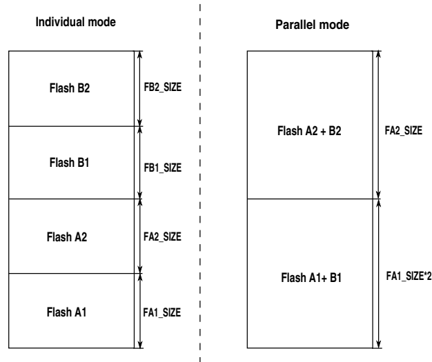
Figure 27-4. Flash memory map in individual and parallel mode
