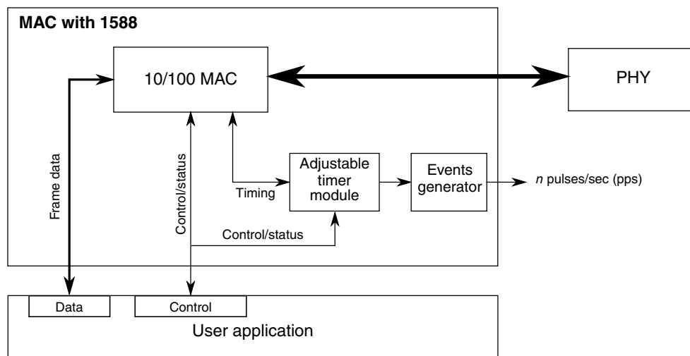
Figure 41-9. IEEE 1588 functions overview
