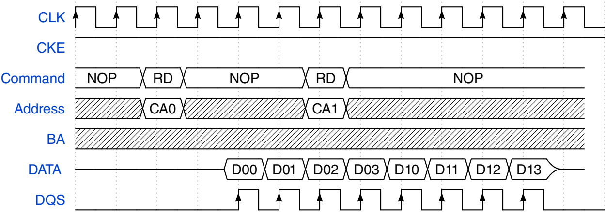
Figure 25-16. SDRAM Read-to-Read access (CL=2)
