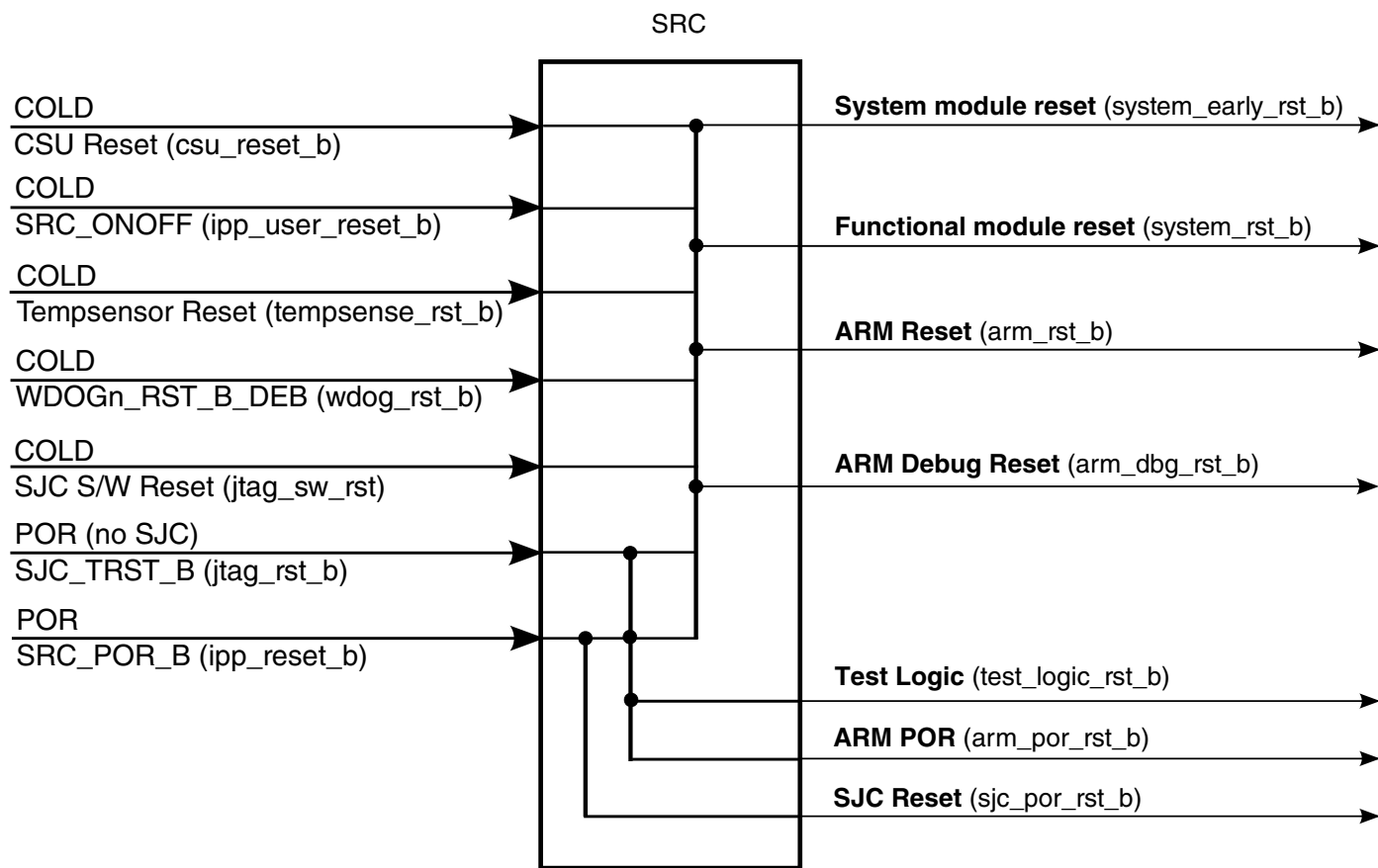
Figure 21-5. SRC inputs and outputs
