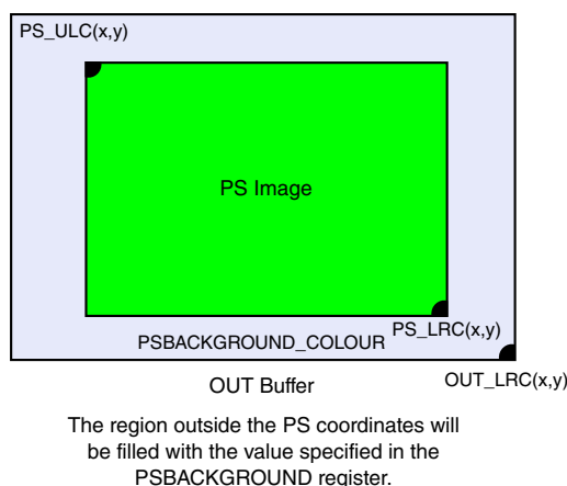
Figure 36-19. OUT Buffer
