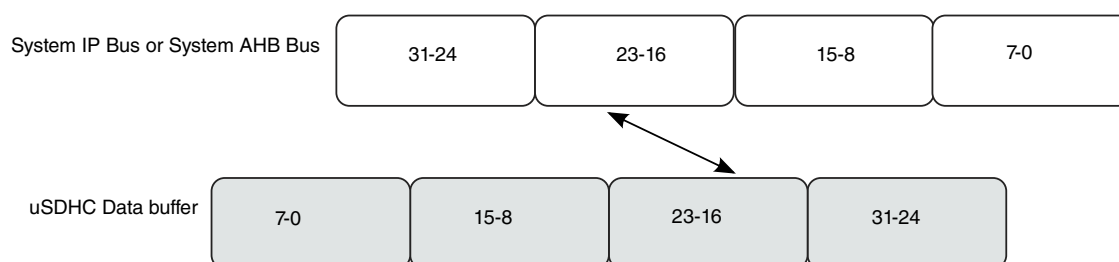
Figure 26-4. Data Swap between System Bus and uSDHC Data Buffer in Byte Little Endian Mode
