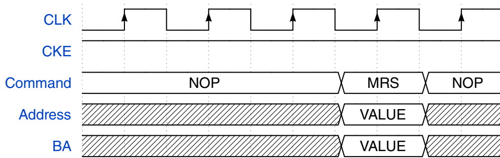
Figure 25-5. IP command - SDRAM MODE REGISTER SET
