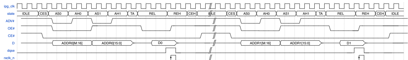
Figure 25-49. Flash Read in ASYNC mode (AADM)
