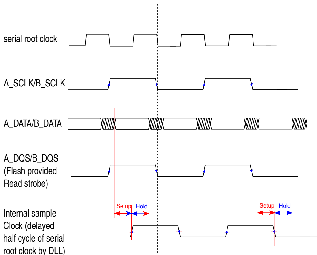
Figure 27-32. Input Timing 2 for Flash provided read strobe in DDR mode
