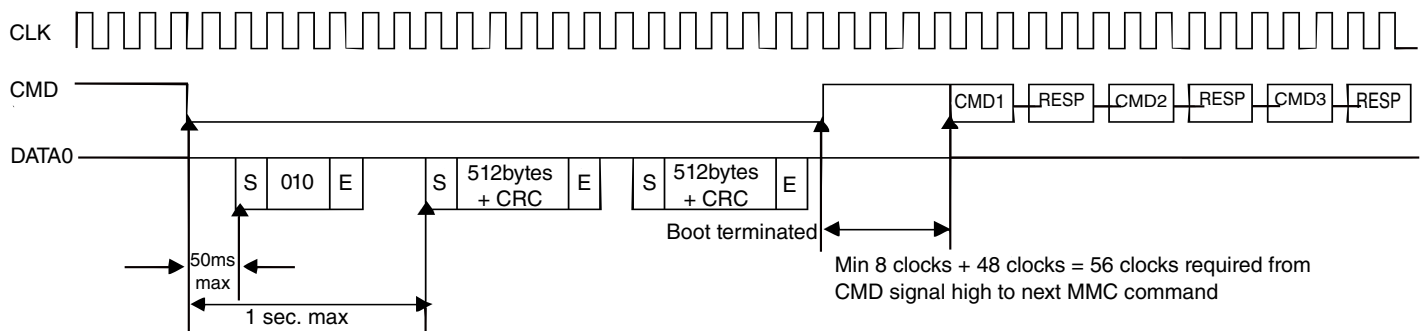
Figure 26-16. MultiMediaCard state diagram (normal boot mode)
