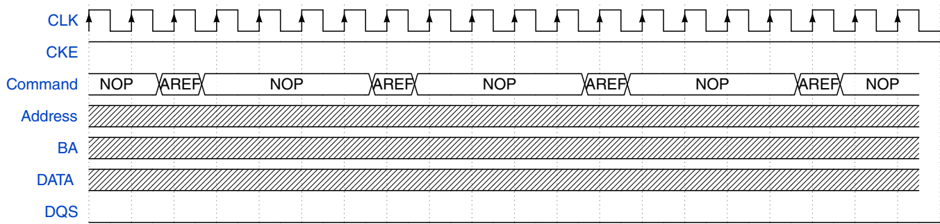
Figure 25-25. Refresh command - SDRAM Auto Refresh
