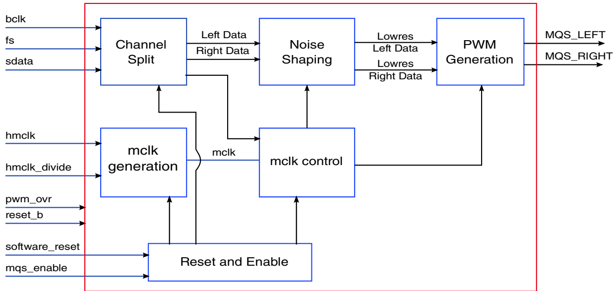
Figure 39-1. Block Diagram
