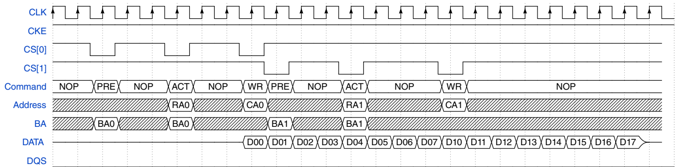
Figure 25-14. AXI command - Pipelined SDRAM Write
