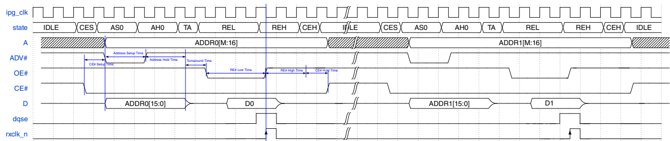
Figure 25-53. SRAM Read in ASYNC mode (ADMUX)
