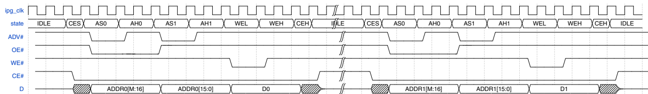
Figure 25-51. Flash Write in ASYNC mode (AADM)
