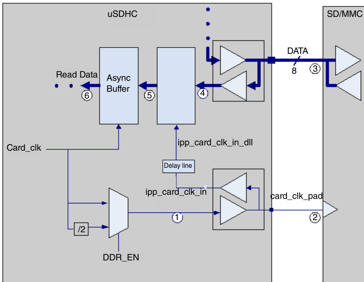
Figure 26-20. DLL(Delay Line) in Read Path
