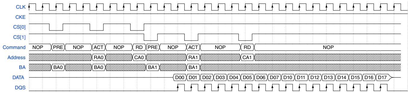
Figure 25-13. AXI command - Pipelined SDRAM Read
