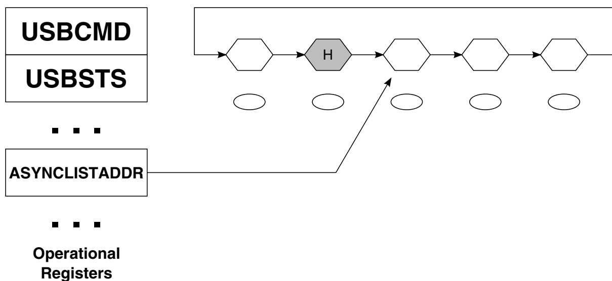
Figure 42-7. General Format of Asynchronous Schedule List
