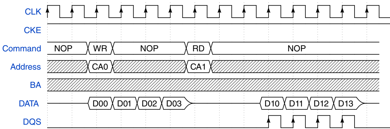
Figure 25-24. SDRAM Write-to-Read access (CL=3)
