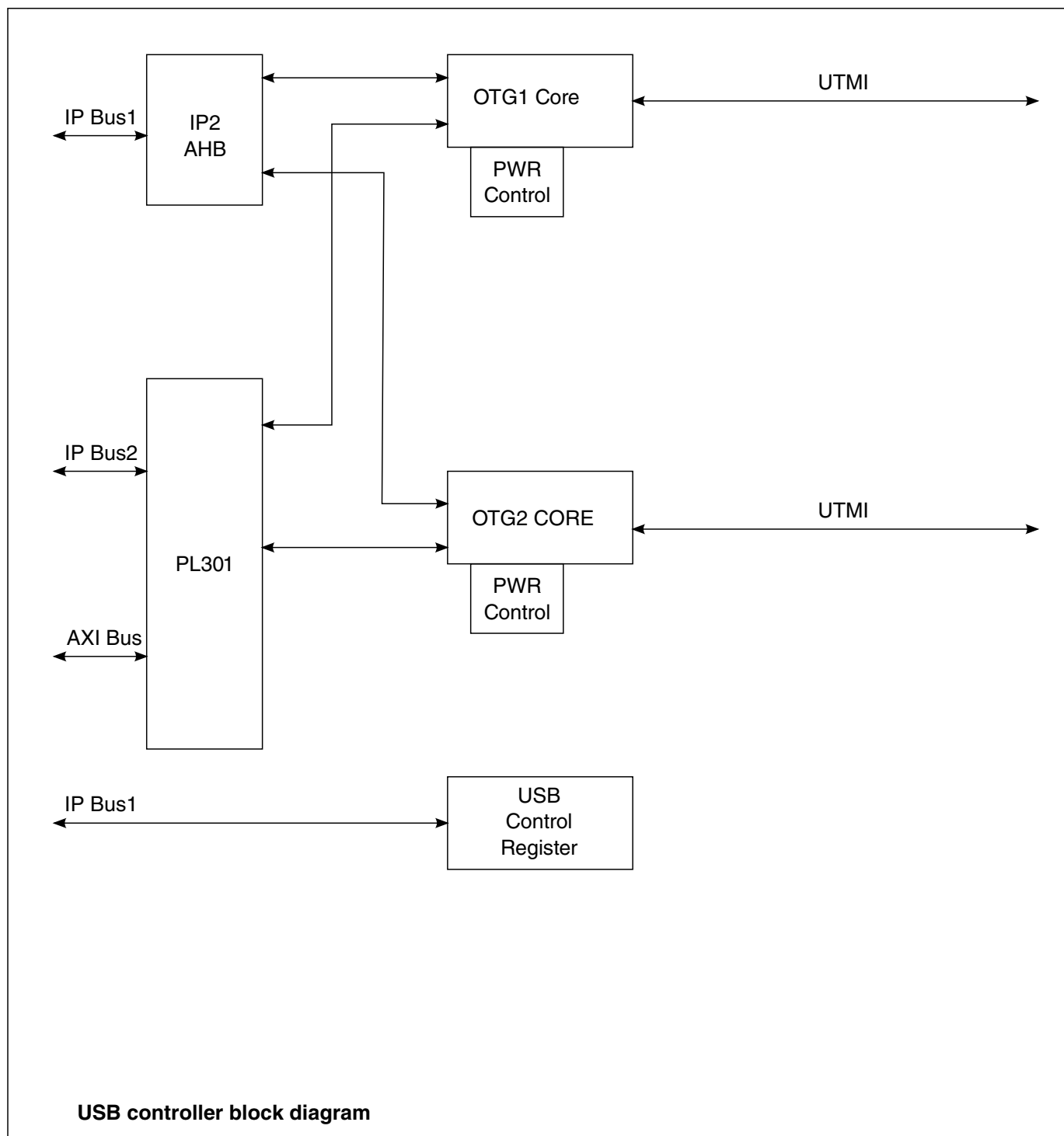
Figure 42-1. USB block diagram
