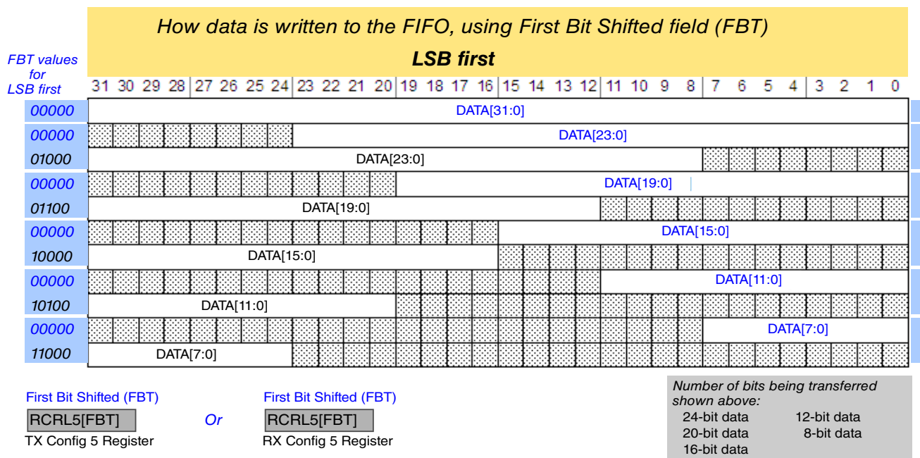
Figure 38-2. SAI first bit shifted, LSB first
