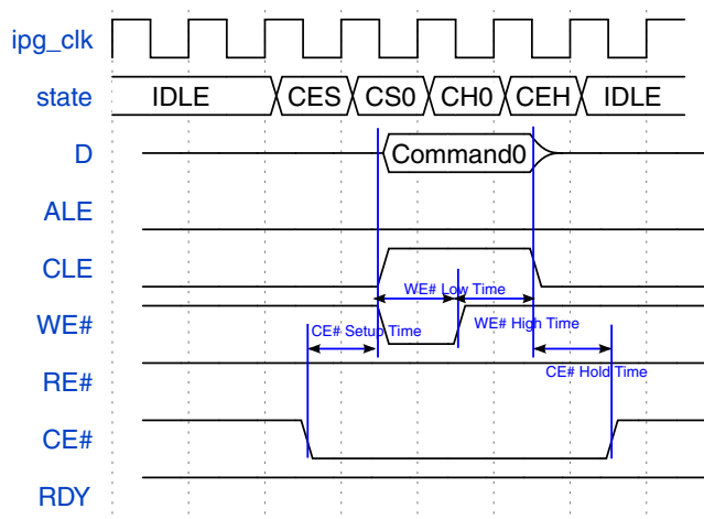
Figure 25-34. NAND Flash access command type - Command Phase Only
