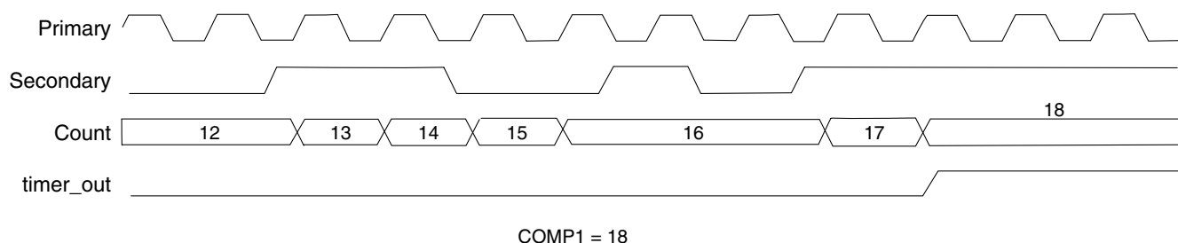
Figure 53-4. Triggered Count Mode 1 (CTRL[LENGTH]=0)
