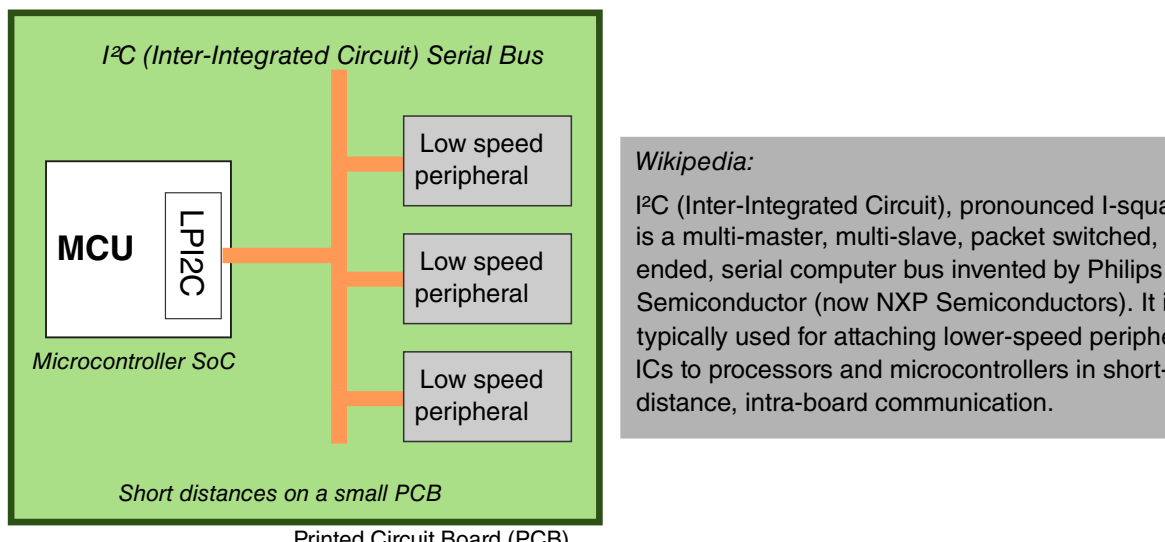
Figure 46-1. I²C bus connects MCU to low speed peripherals on PCB
