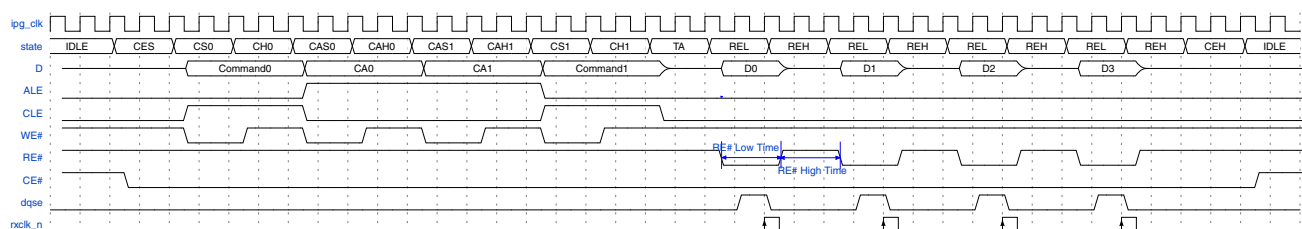
Figure 25-44. NAND Flash access command type - Command + Address + Command + Read Phase
