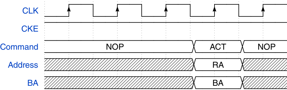
Figure 25-8. IP command - SDRAM ACTIVE
