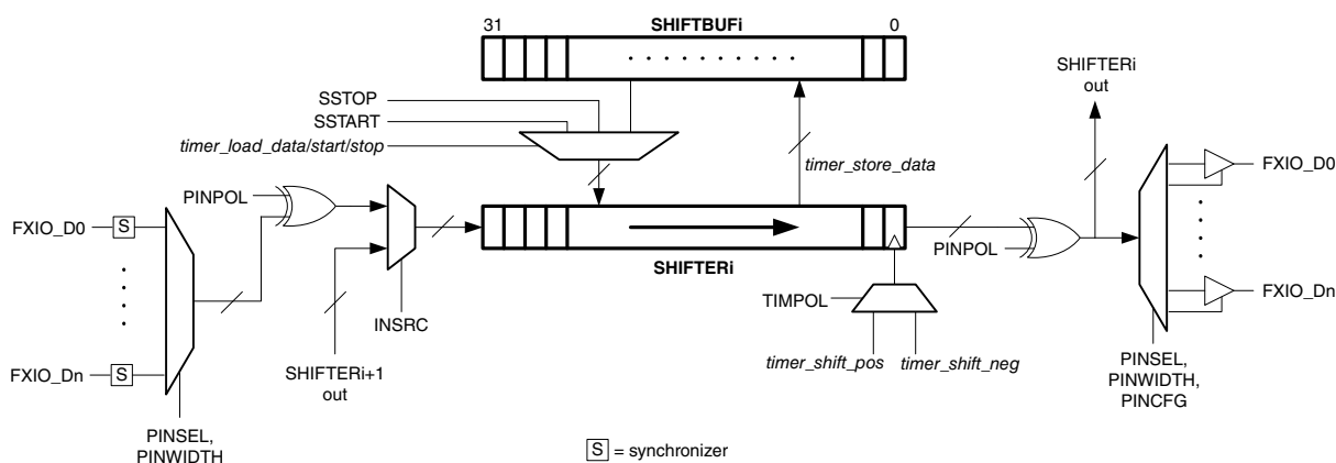
Figure 49-2. Shifter Microarchitecture
