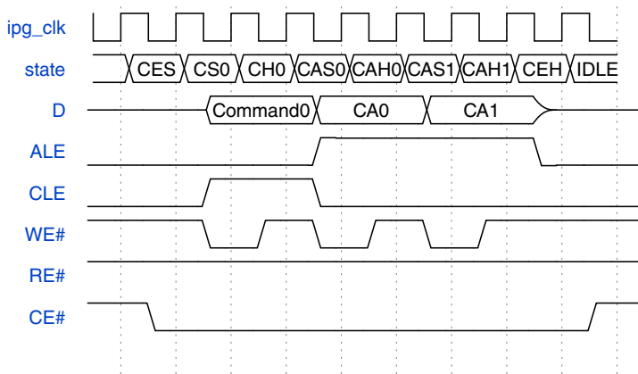
Figure 25-29. NAND Flash access Address type - Two Byte Column Address
