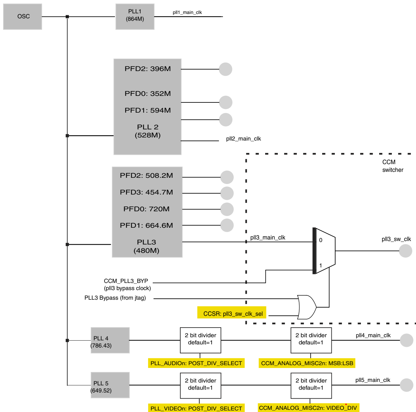
Figure 14-4. Switcher clock generation
