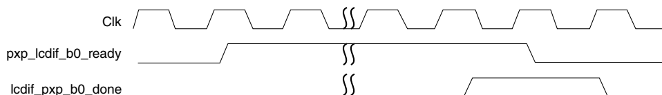
Figure 36-16. Buffer Sharing Protocol
