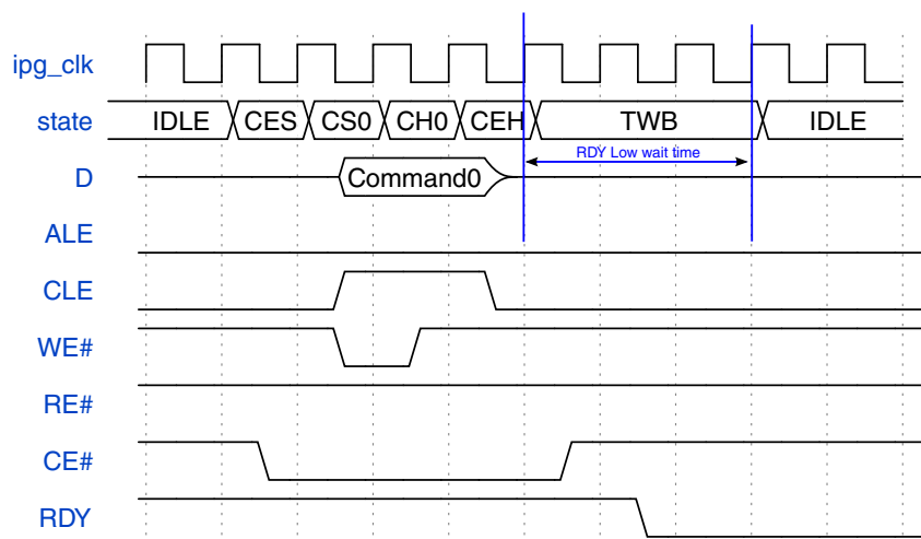
Figure 25-35. NAND Flash access command type - Command + Wait Phase
