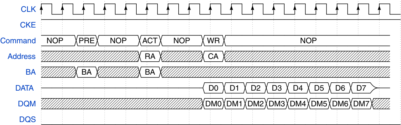
Figure 25-12. AXI command - SDRAM Write
