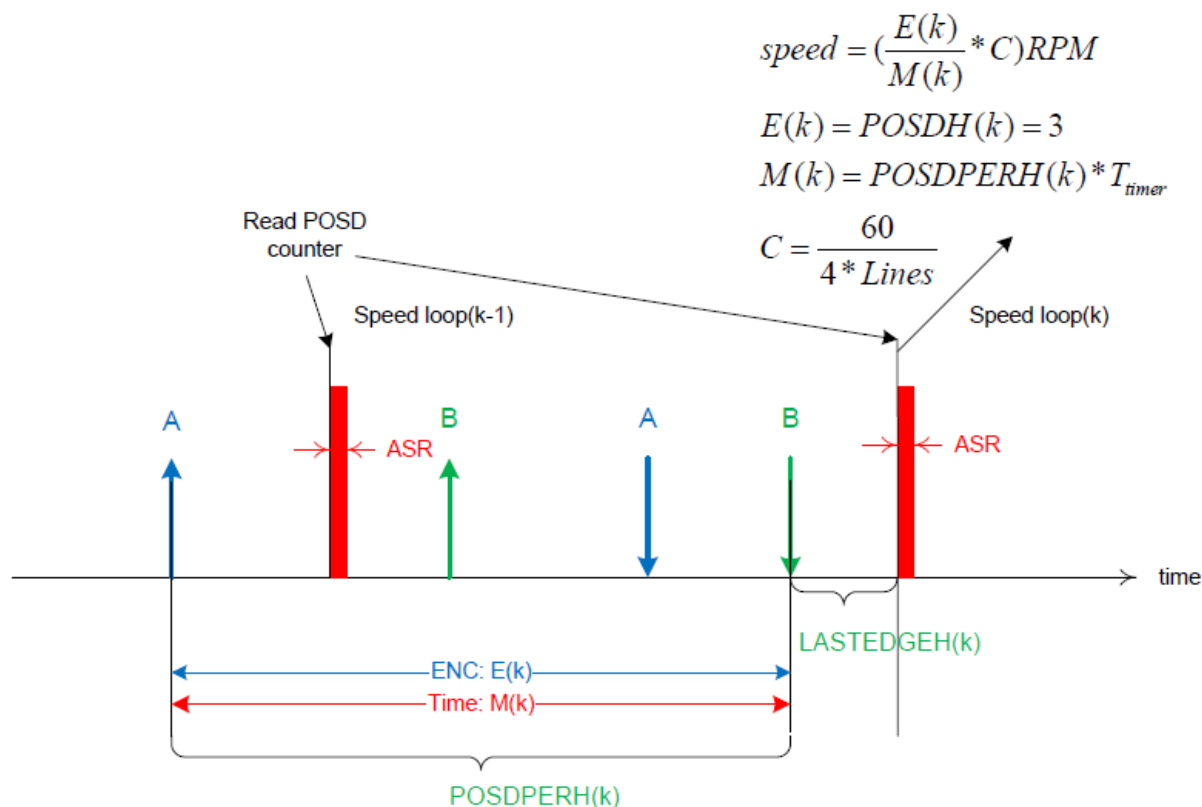
Figure 55-5. High speed measurement with method
