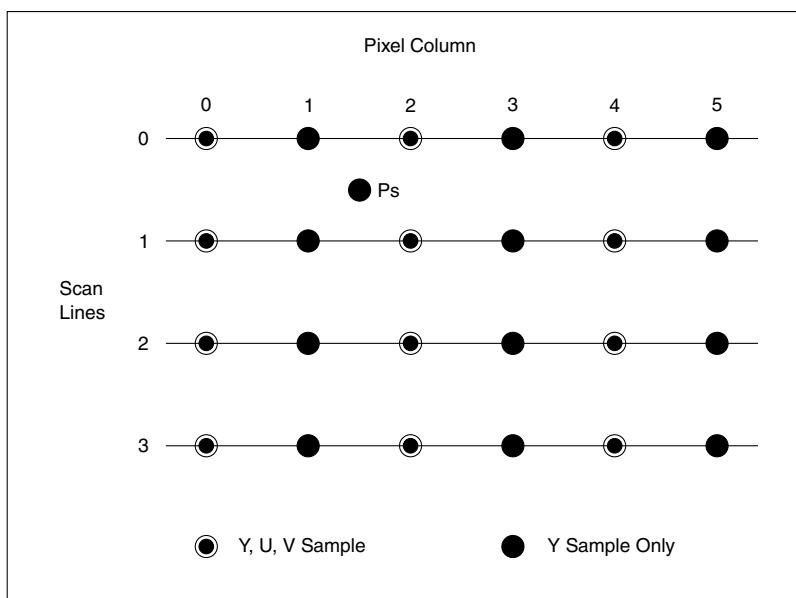
Figure 36-6. YUV Sample Positioning, 4:2:2
