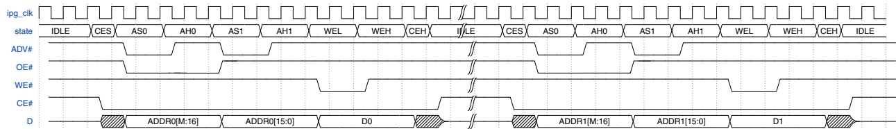
Figure 25-56. SRAM Write in ASYNC mode (AADM)
