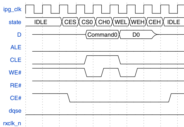
Figure 25-41. NAND Flash access command type - Command + Write Phase
