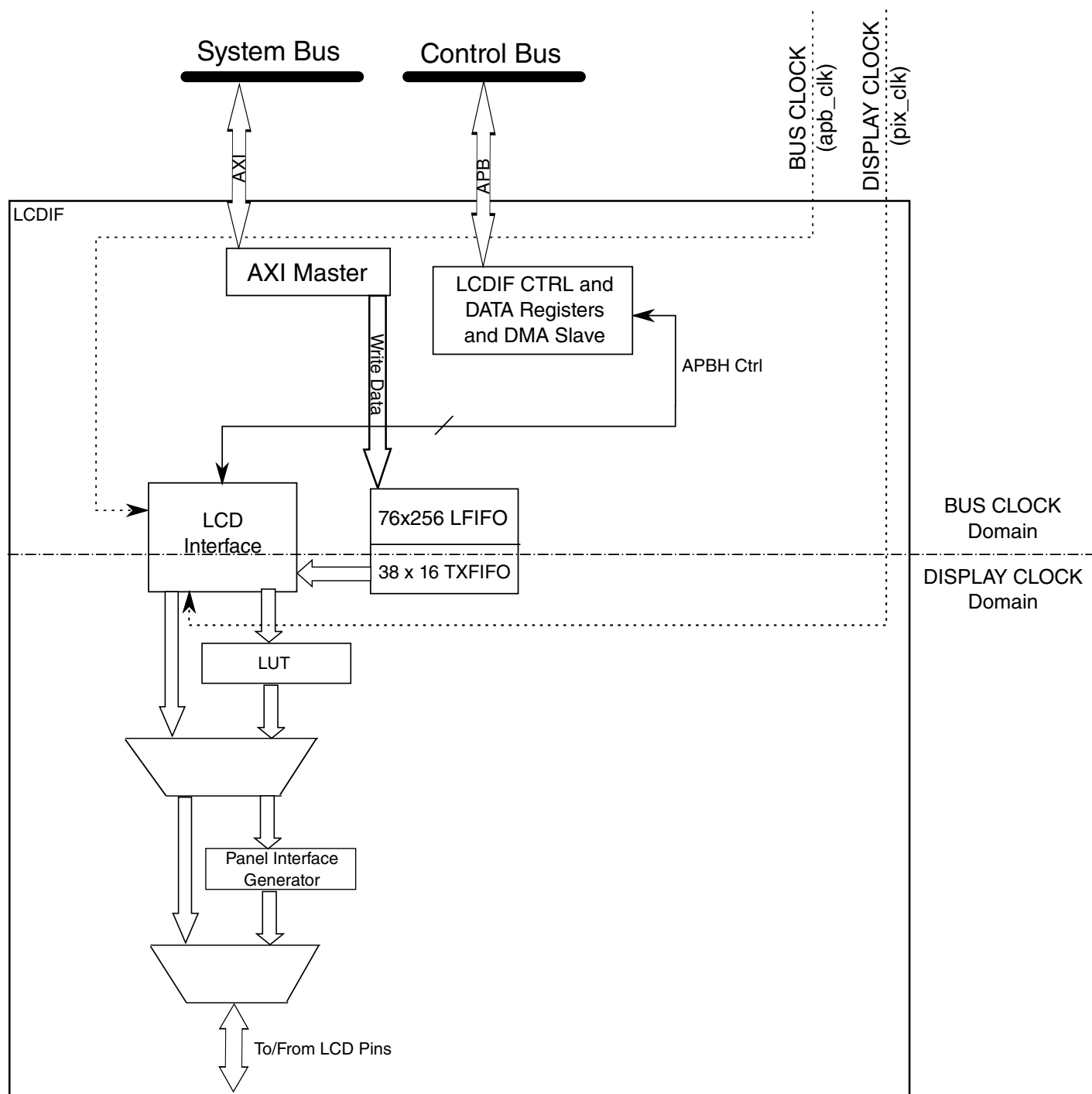
Figure 35-1. Top-Level Block Diagram of LCDIF subsystem
