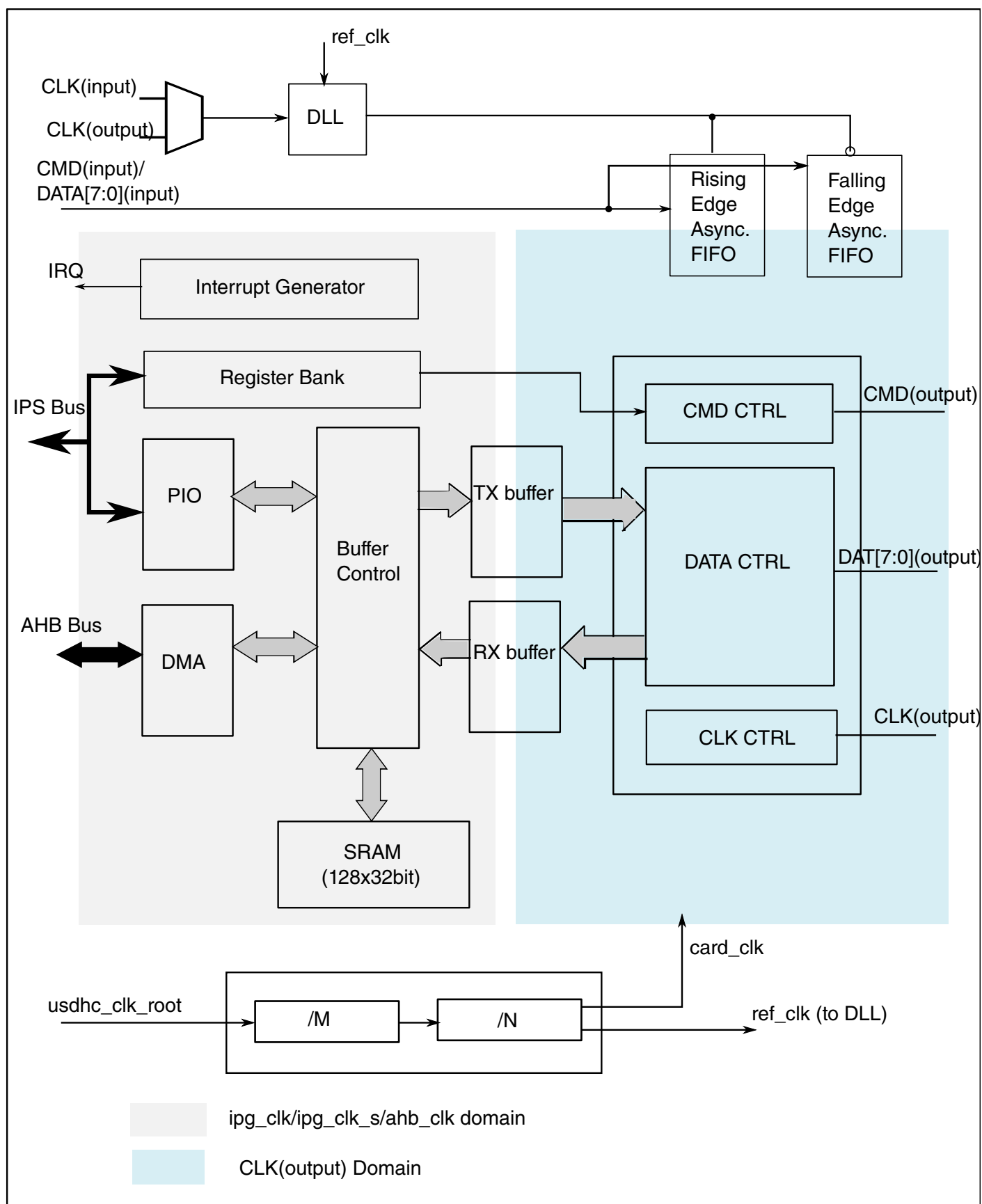
Figure 26-2. ultra Secure Digital Host Controller Block Diagram
