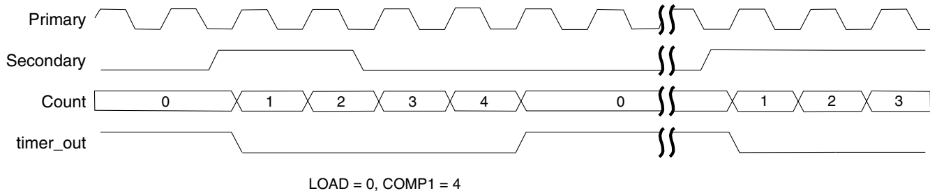
Figure 53-6. One-Shot Mode (CTRL[LENGTH]=1)
