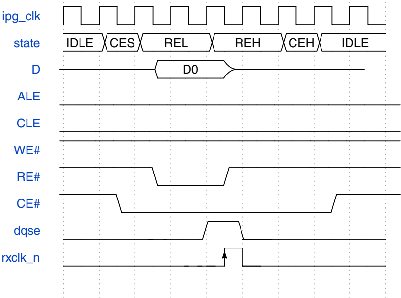
Figure 25-42. NAND Flash access command type - Read Phase Only
