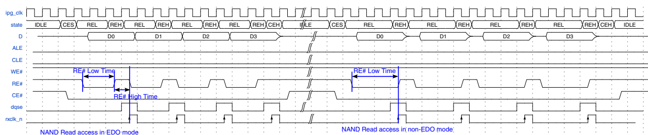
Figure 25-46. NAND Flash Read Access in EDO or non-EDO mode
