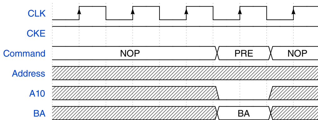
Figure 25-6. IP command - SDRAM PRECHARGE
