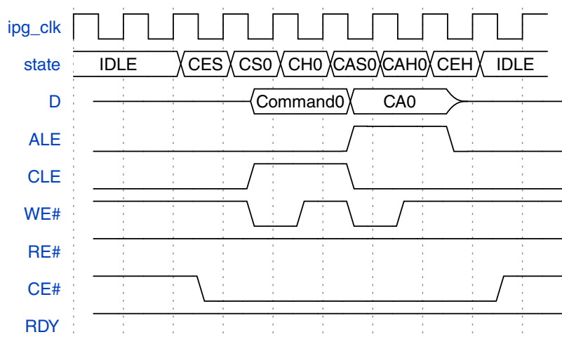
Figure 25-36. NAND Flash access command type - Command + Address Phase
