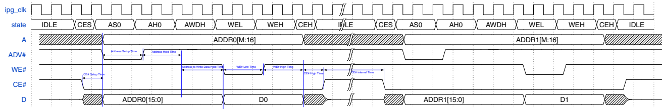
Figure 25-50. Flash Write in ASYNC mode (ADMUX)
