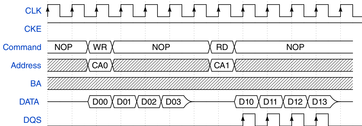
Figure 25-22. SDRAM Write-to-Read access (CL=1)
