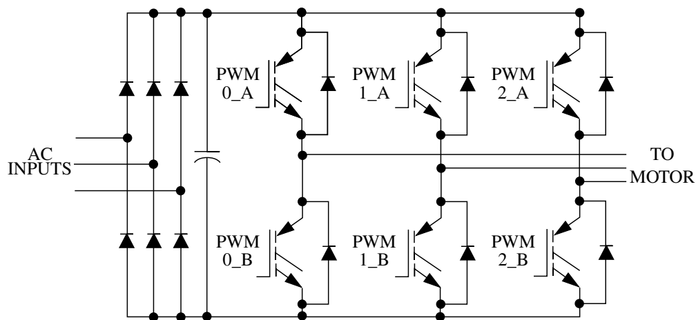
Figure 54-19. Typical 3 Phase AC Motor Drive
