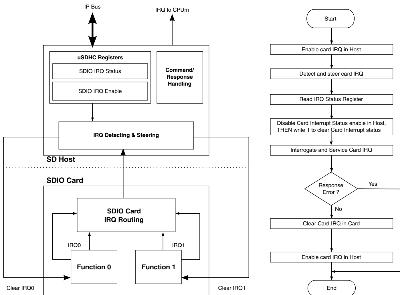
Figure 26-15. Card Interrupt Scheme and Card Interrupt Detection and Handling Procedure
