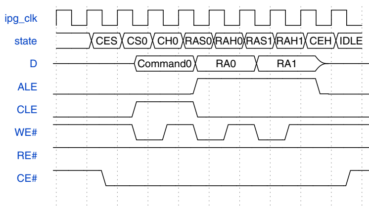
Figure 25-31. NAND Flash access Address type - Two Byte Row Address
