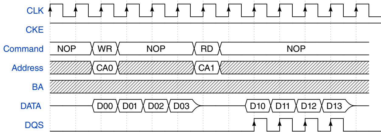
Figure 25-23. SDRAM Write-to-Read access (CL=2)
