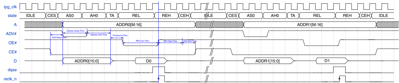
Figure 25-48. Flash Read in ASYNC mode (ADMUX)
