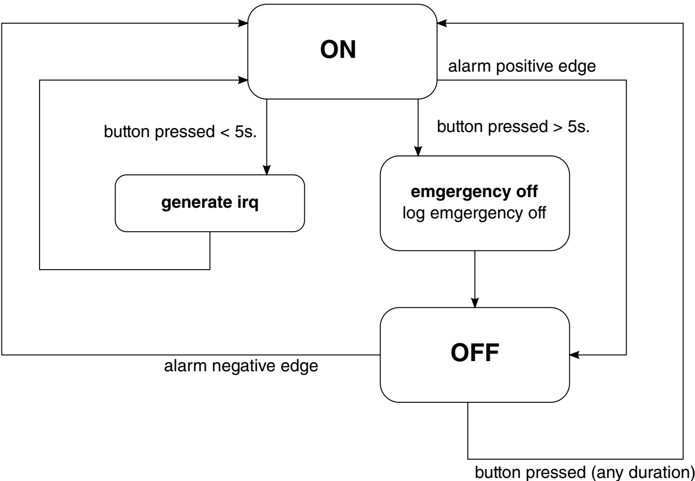
Figure 21-4. FSM
