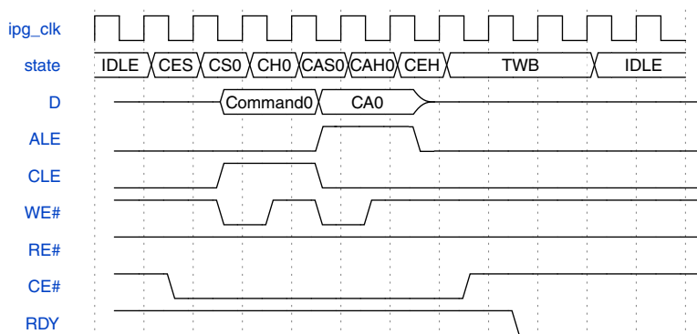
Figure 25-37. NAND Flash access command type - Command + Address + Wait Phase
