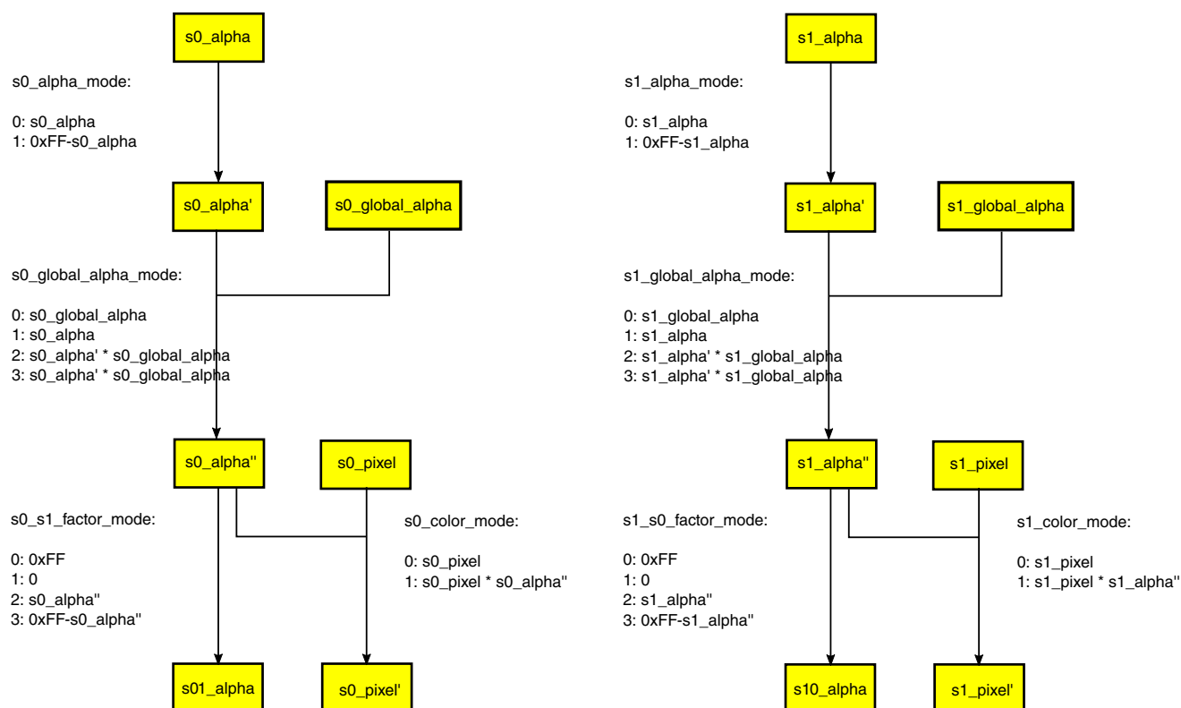
Figure 36-9. Porter-Duff Alpha Blend
