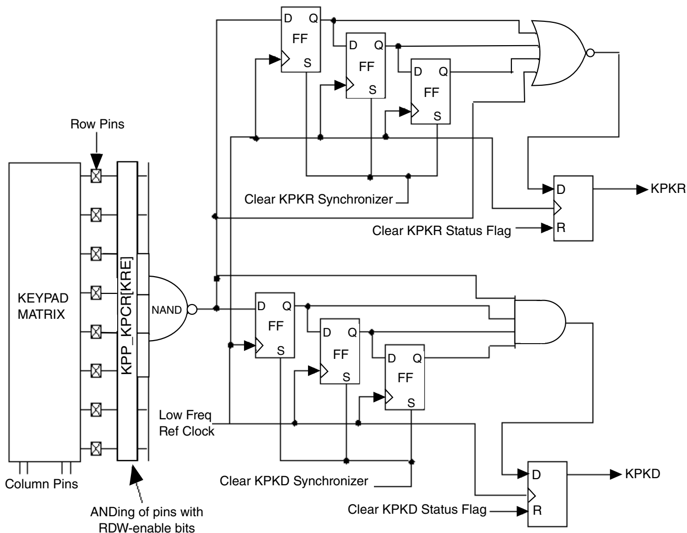
Figure 45-2. Keypad Synchronizer Functional Diagram
