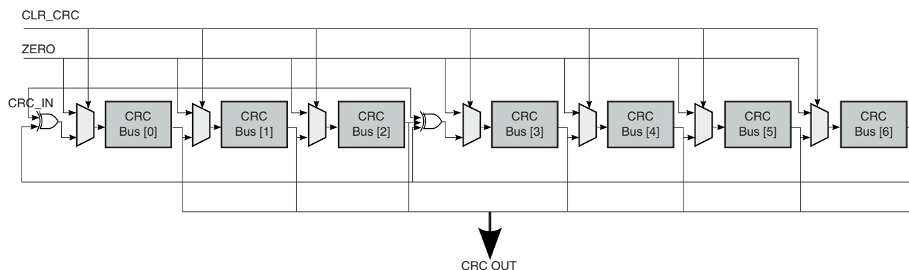
Figure 26-13. Command CRC Shift Register
