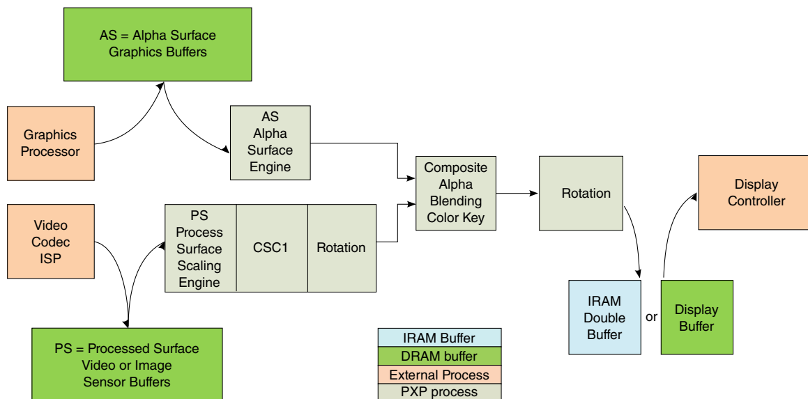
Figure 36-1. PXP Architecture
