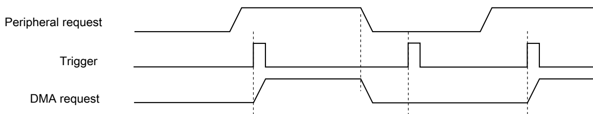
Figure 5-4. DMAMUX channel triggering: ignored trigger
