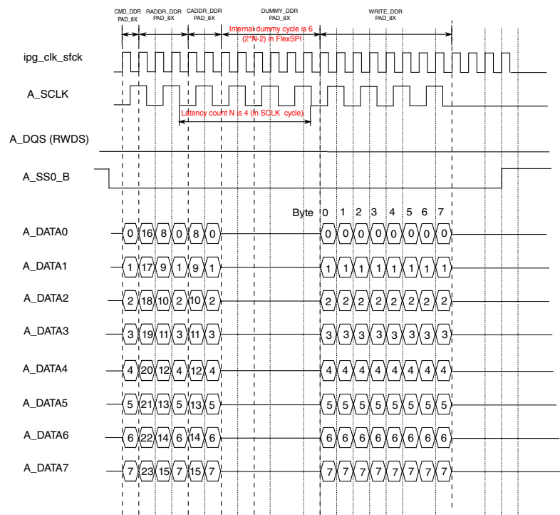
Figure 27-11. HyperBus device write transaction with single latency count
