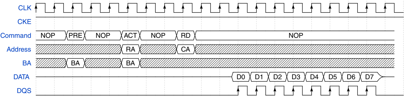
Figure 25-11. AXI command - SDRAM Read
