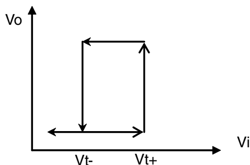
Figure 12-4. Schmitt trigger transfer characteristic
