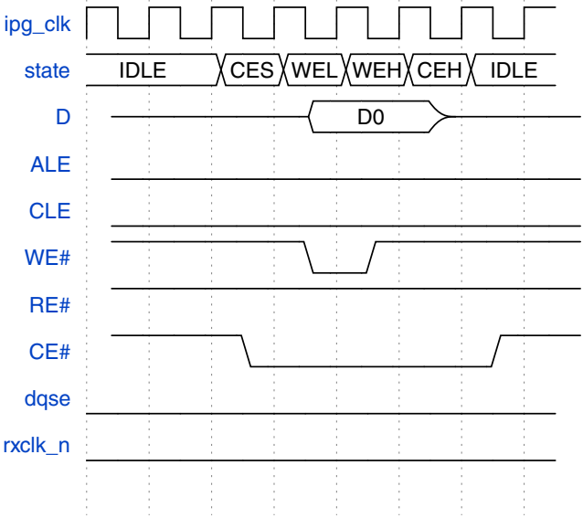
Figure 25-43. NAND Flash access command type - Write Phase Only
