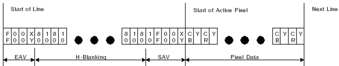
Figure 34-3. CCIR656 General Line Timing
