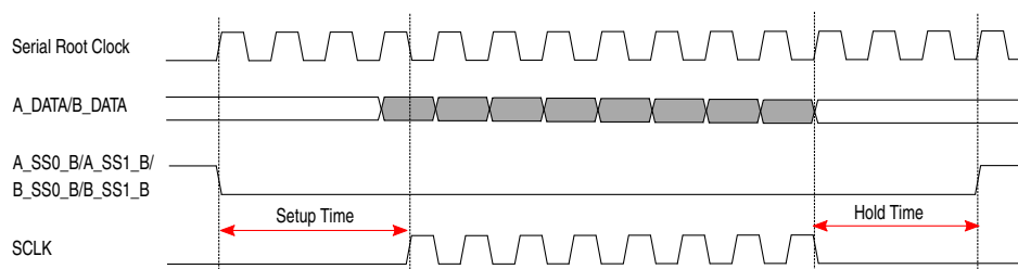
Figure 27-26. Chip selection output timing for SDR sequence
