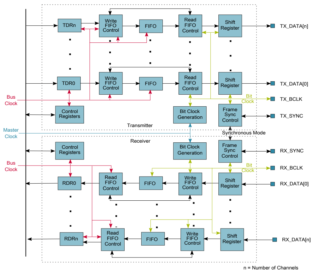
Figure 38-1. I²S/SAI block diagram
