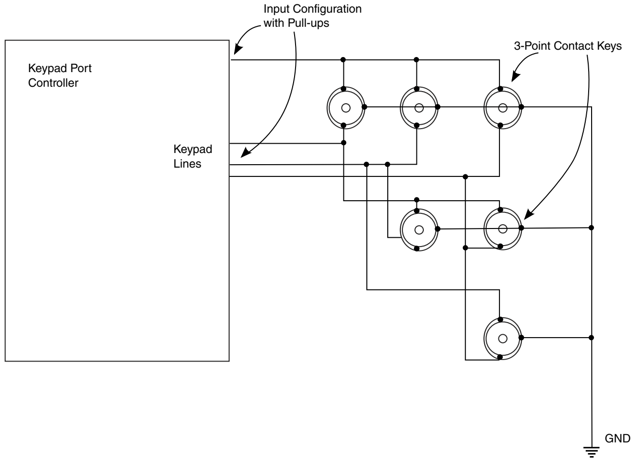
Figure 45-7. KPP Interface with 3-point Contact Key Matrix (Simplified View)
