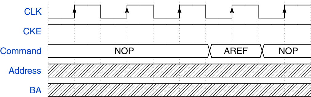
Figure 25-4. IP command - SDRAM Auto Refresh
