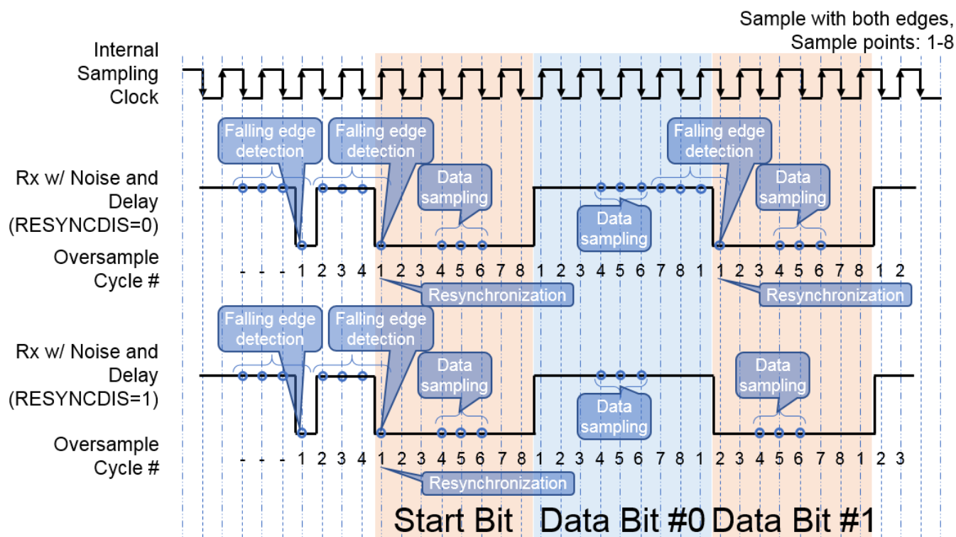
Figure 48-5. LPUART resynchronization
