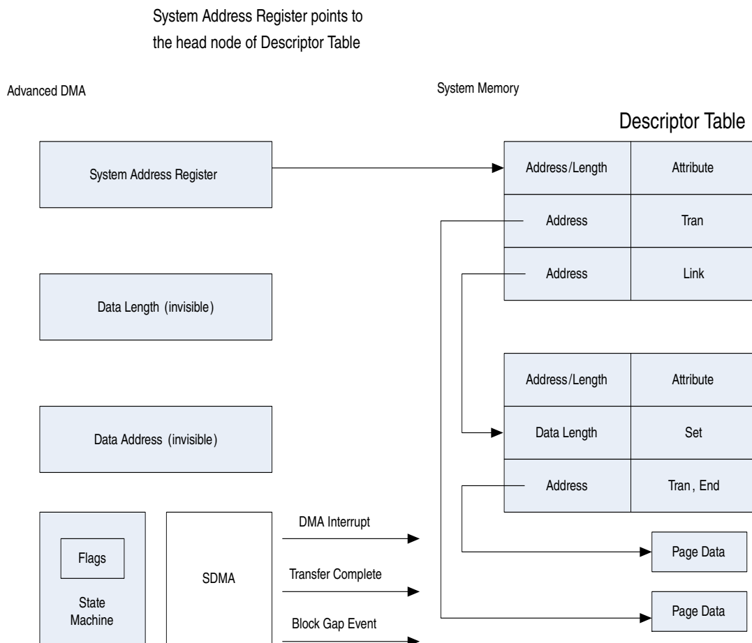
Figure 26-9. Concept and Access Method of ADMA1 Descriptor Table
