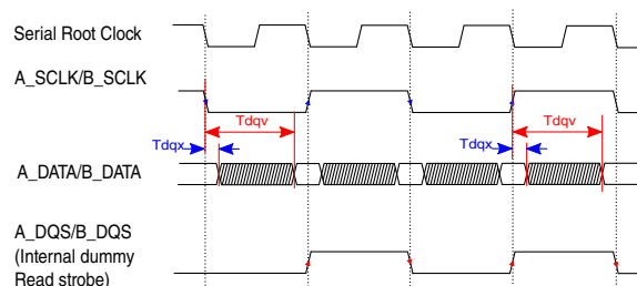
Figure 27-30. Input Timing for sampling with dummy read strobe in DDR mode
