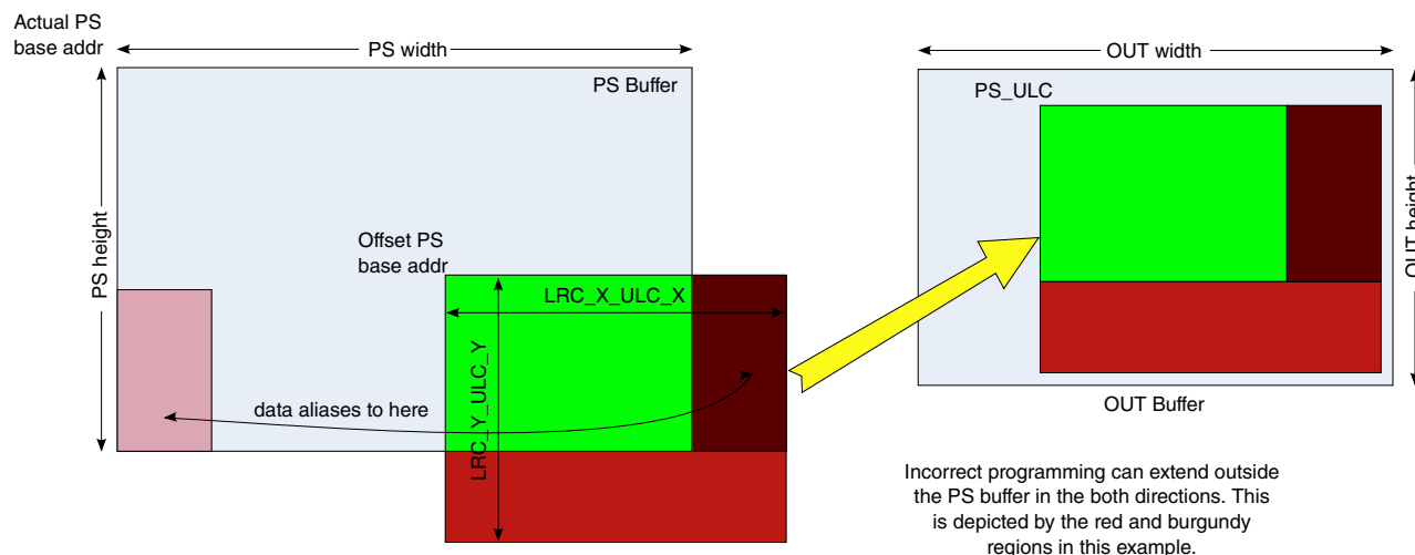
Figure 36-21. Example with Invalid Parameters
