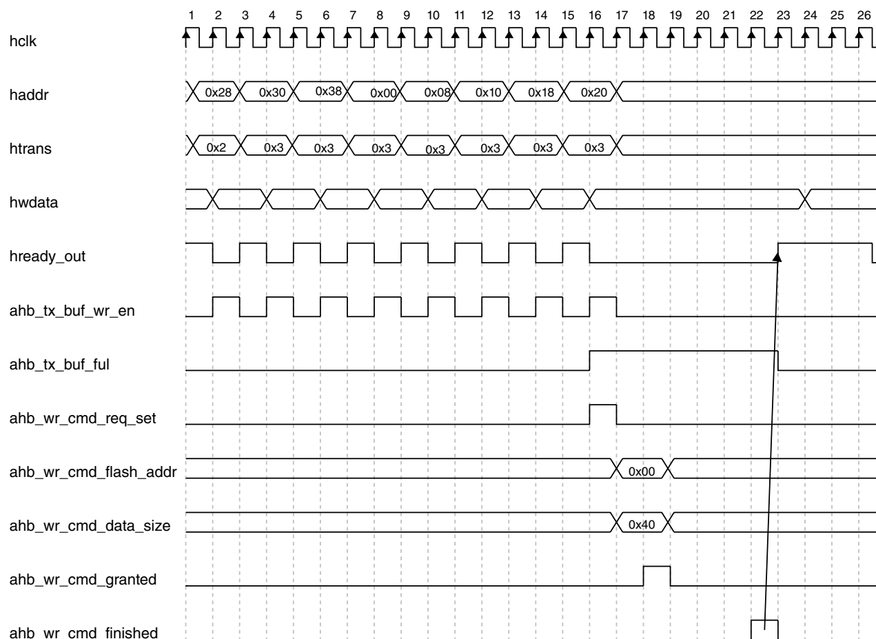
Figure 27-20. AHB write access (WRAP8/64bit/Non-Bufferable)
