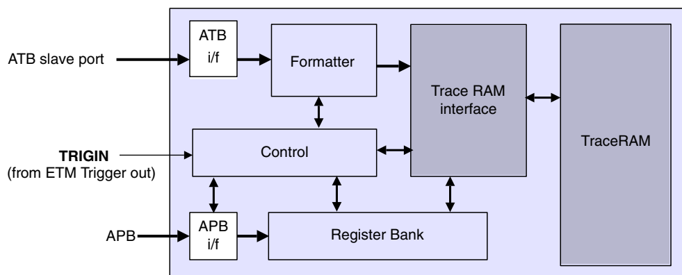
Figure 8-1. ETB Block Diagram
