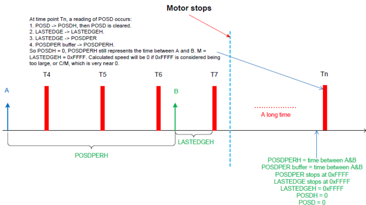
Figure 55-12. Speed measurement at time point Tn
