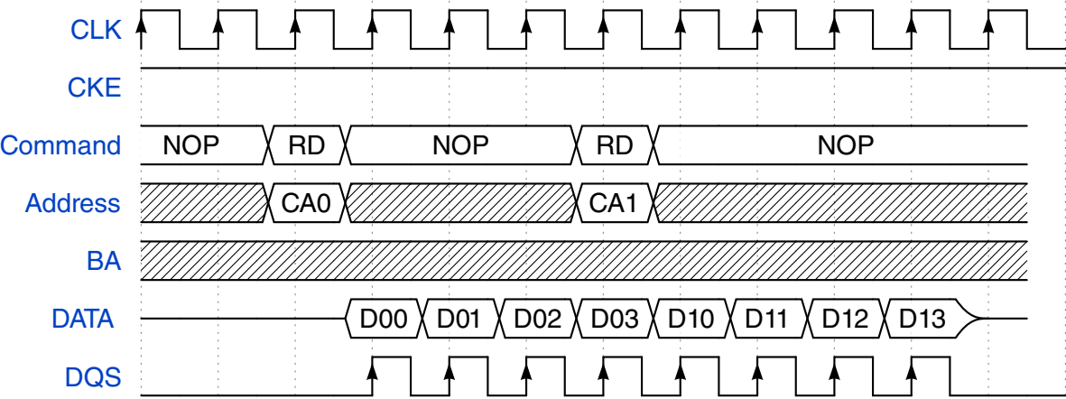
Figure 25-15. SDRAM Read-to-Read access (CL=1)
