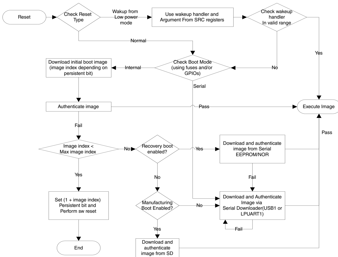
Figure 9-1. Boot flow
