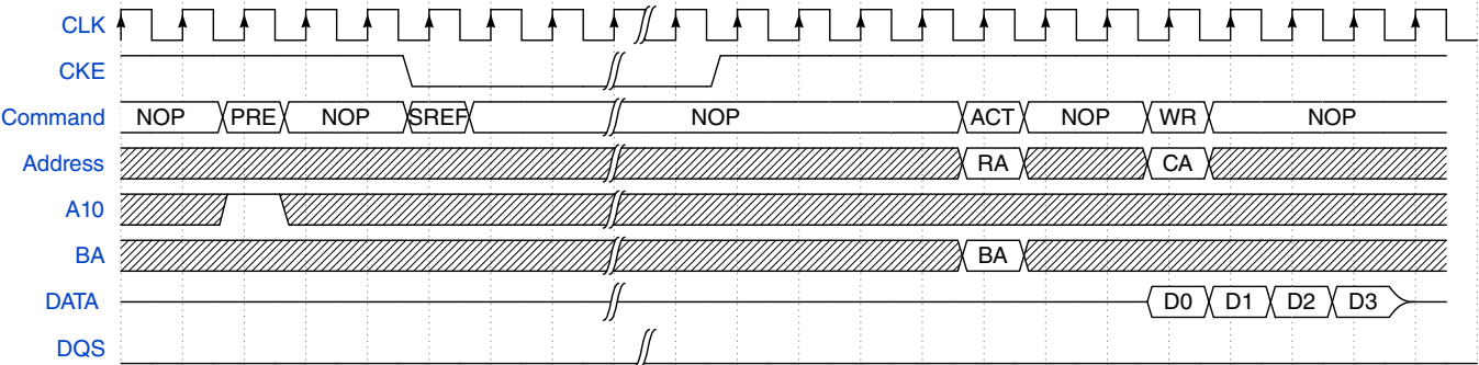
Figure 25-3. IP command - SDRAM Self Refresh
