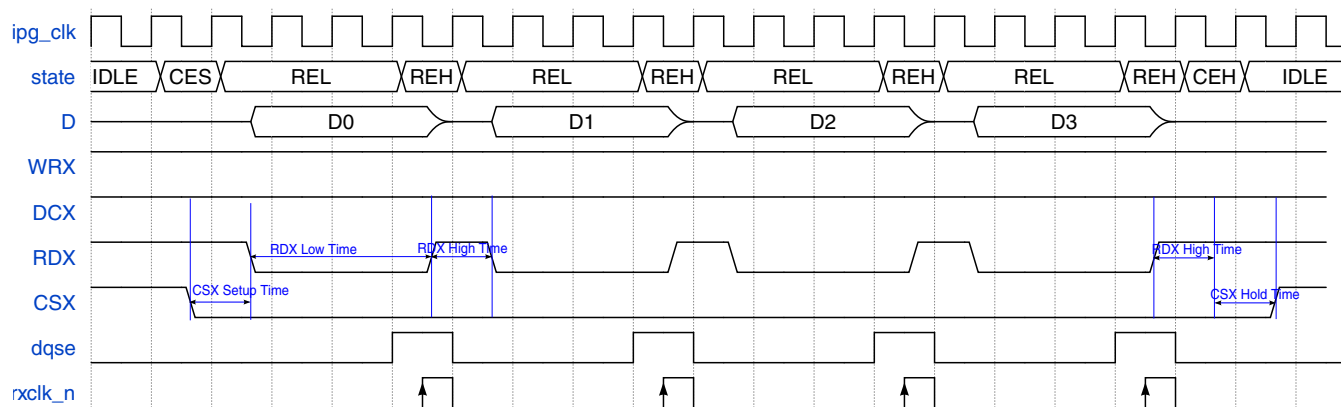
Figure 25-58. DBI Read Operation
