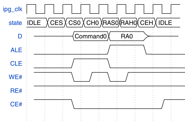
Figure 25-30. NAND Flash access Address type - One Byte Row Address
