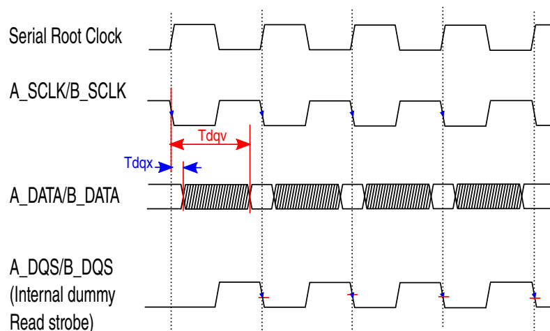
Figure 27-29. Input Timing for sampling with dummy read strobe in SDR mode
