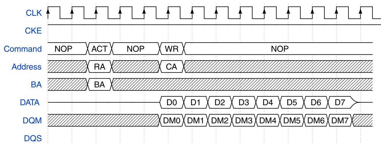
Figure 25-10. IP command - SDRAM WRITE
