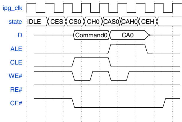
Figure 25-28. NAND Flash access Address type - One Byte Column Address
