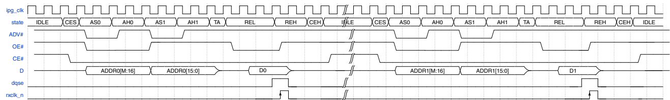
Figure 25-54. SRAM Read in ASYNC mode (AADM)
