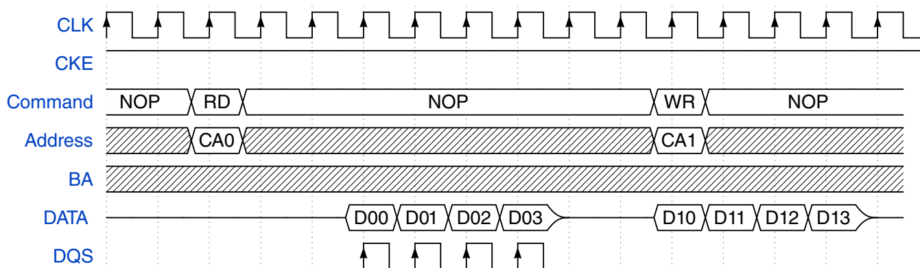
Figure 25-20. SDRAM Read-to-Write access (CL=3)
