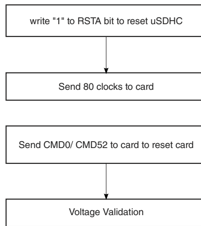
Figure 26-19. Flow Chart for Reset of the uSDHC and SD I/O Card
