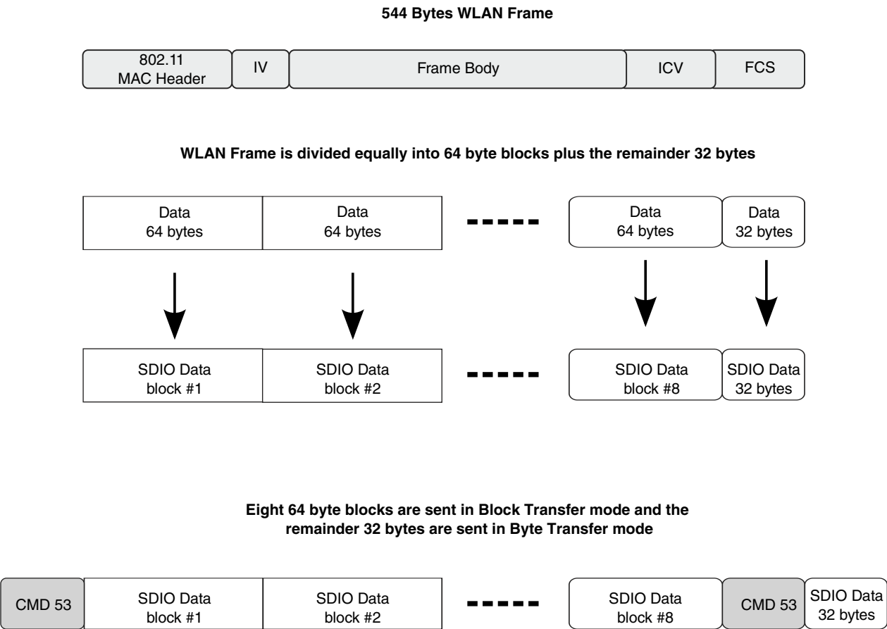
Figure 26-6. Example for Dividing Large Data Transfers
