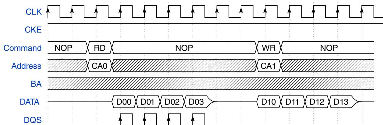
Figure 25-18. SDRAM Read-to-Write access (CL=1)
