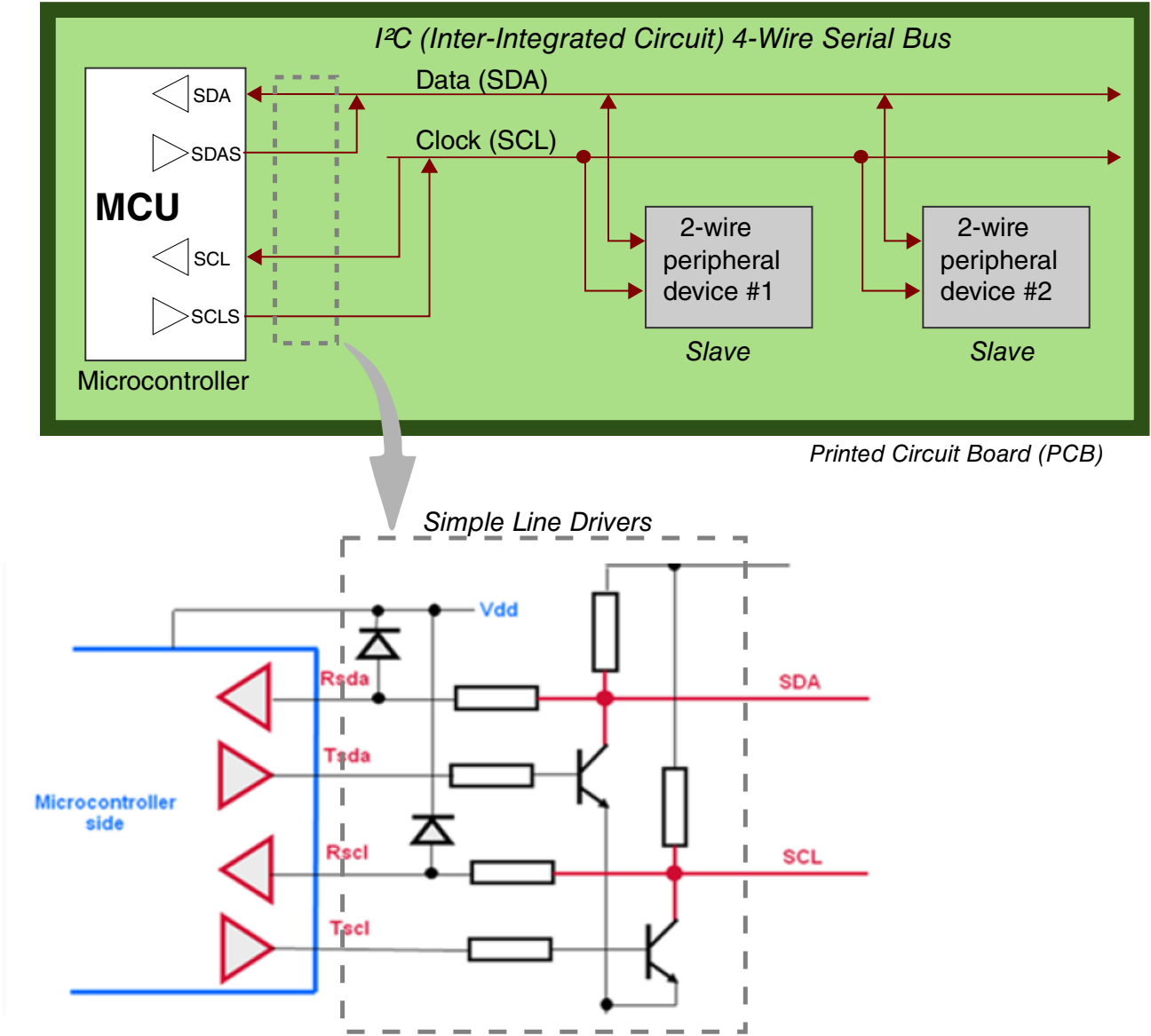
Figure 46-6. 4-Wire scheme
