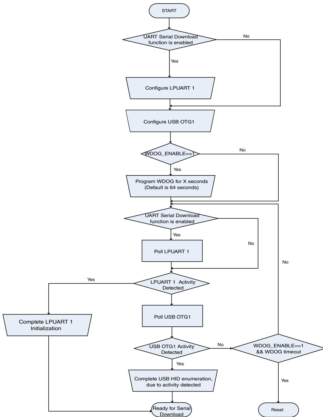
Figure 9-18. Serial Downloader boot flow
