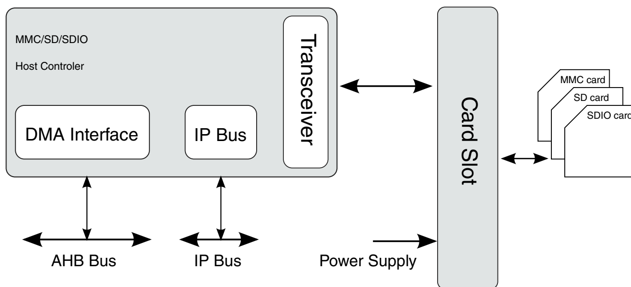
Figure 26-1. System Connection of the uSDHC
