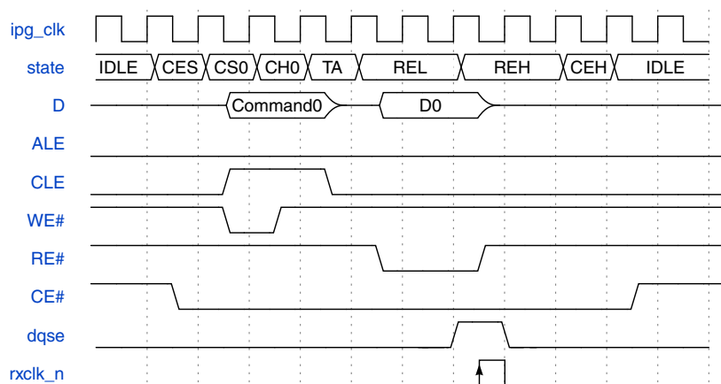
Figure 25-40. NAND Flash access command type - Command + Read Phase
