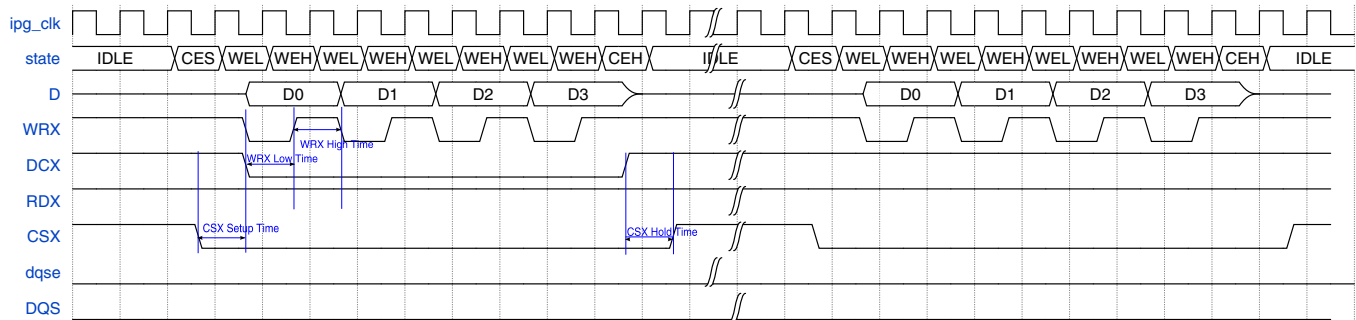
Figure 25-57. DBI Write Operation
