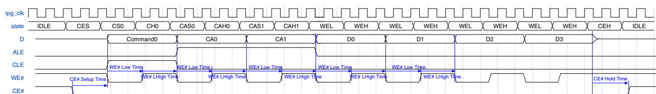
Figure 25-45. NAND Flash access command type - Command + Address + Write Phase
