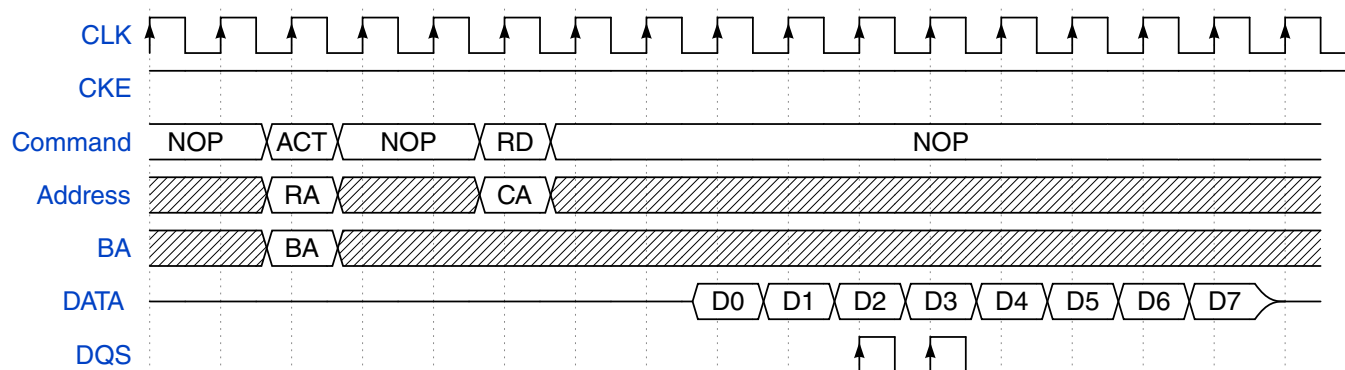
Figure 25-9. IP command - SDRAM READ
