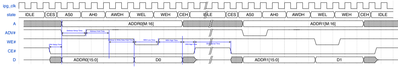
Figure 25-55. SRAM Write in ASYNC mode (ADMUX)
