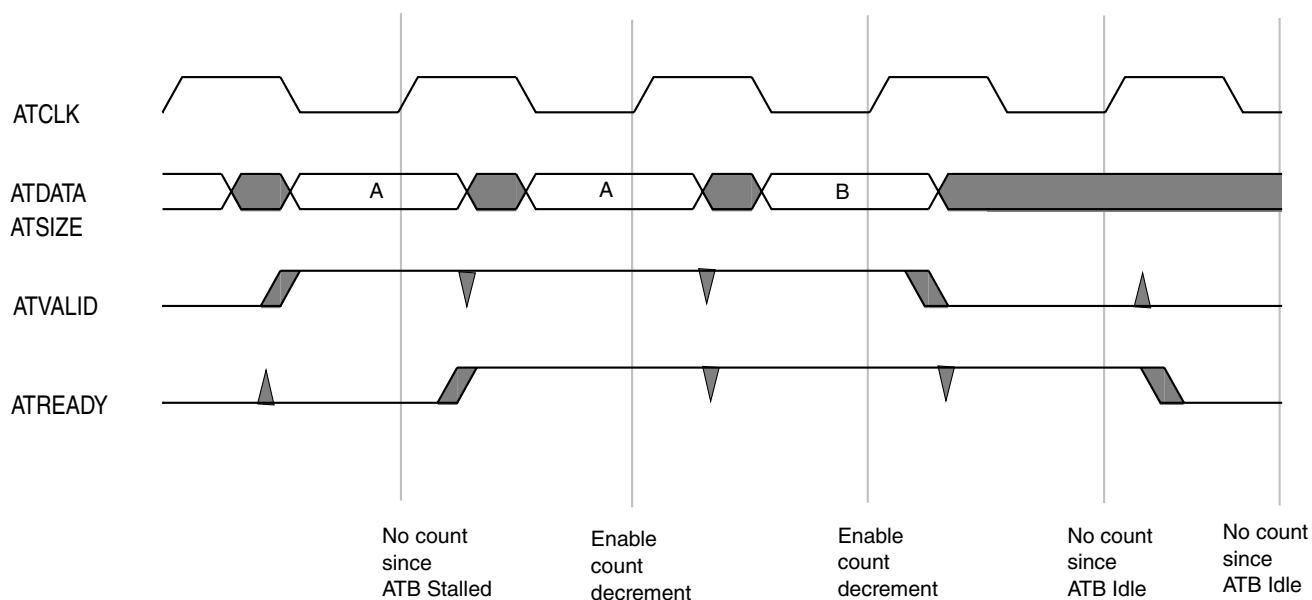
Figure 8-2. Count Decrement Enable
