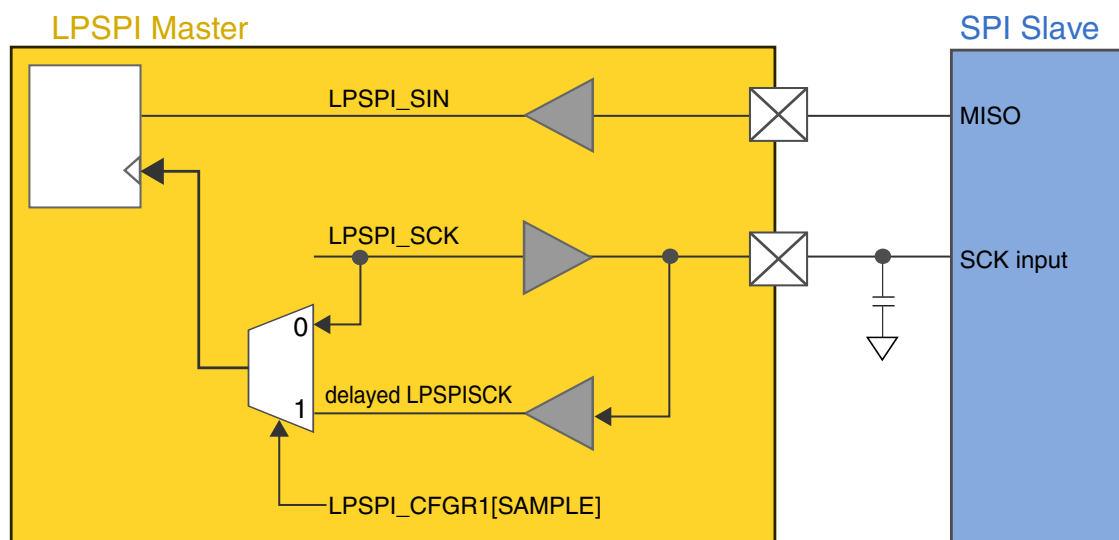
Figure 47-2. Clock Loopback
