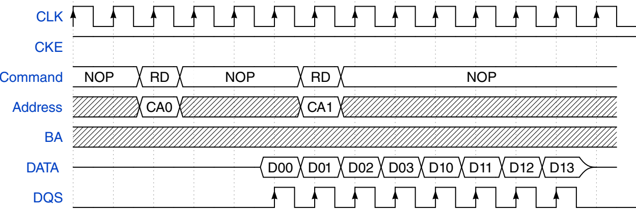
Figure 25-17. SDRAM Read-to-Read access (CL=3)
