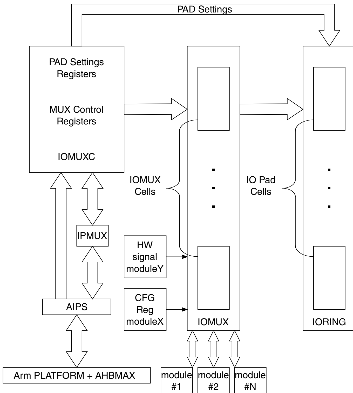
Figure 11-1. IOMUX SoC Level Block Diagram
