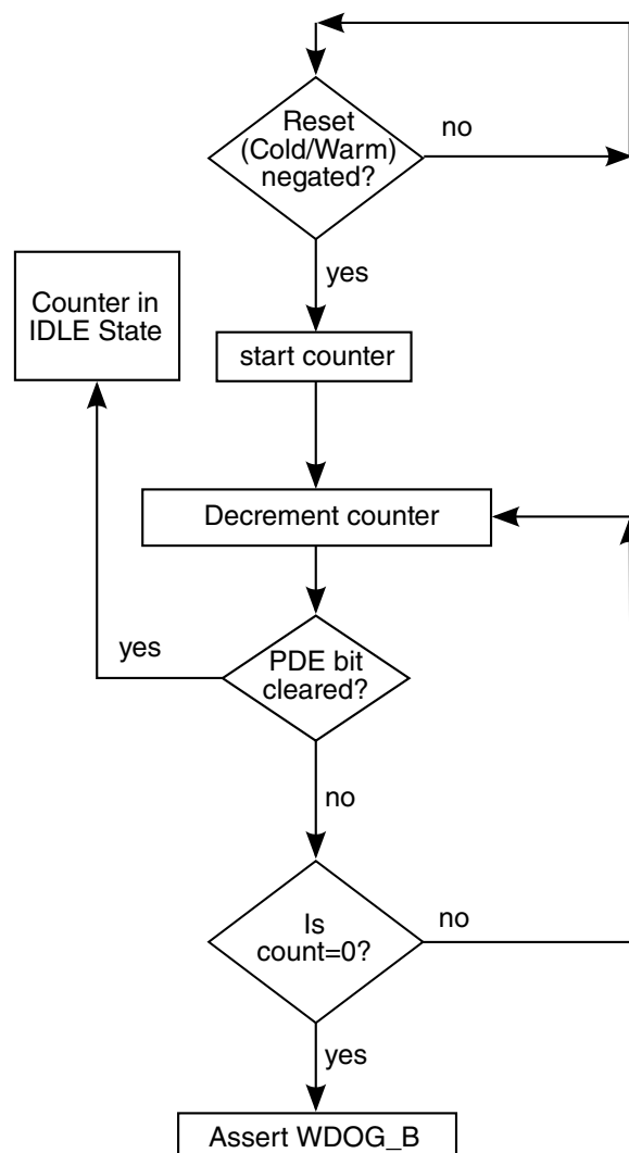
Figure 56-5. Power-Down Counter Flow Diagram
