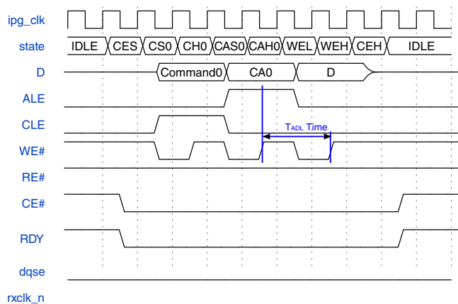
Figure 25-39. NAND Flash access command type - Command + Address + Write Phase
